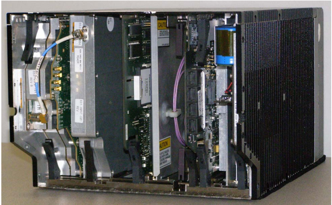
Figure 7 - Front View Assembly Detail
