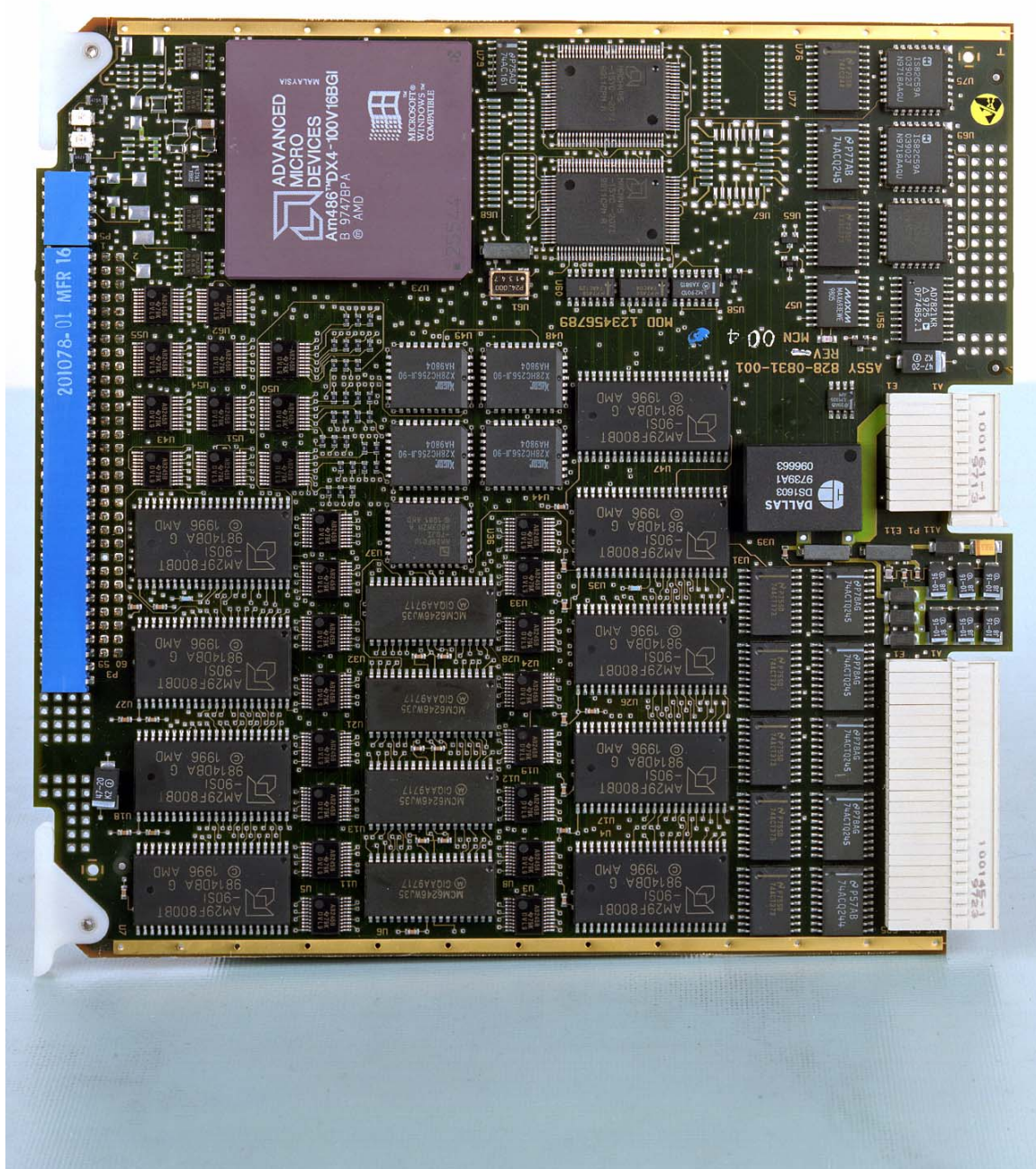
Figure 8-2. System Processor Card Assembly
