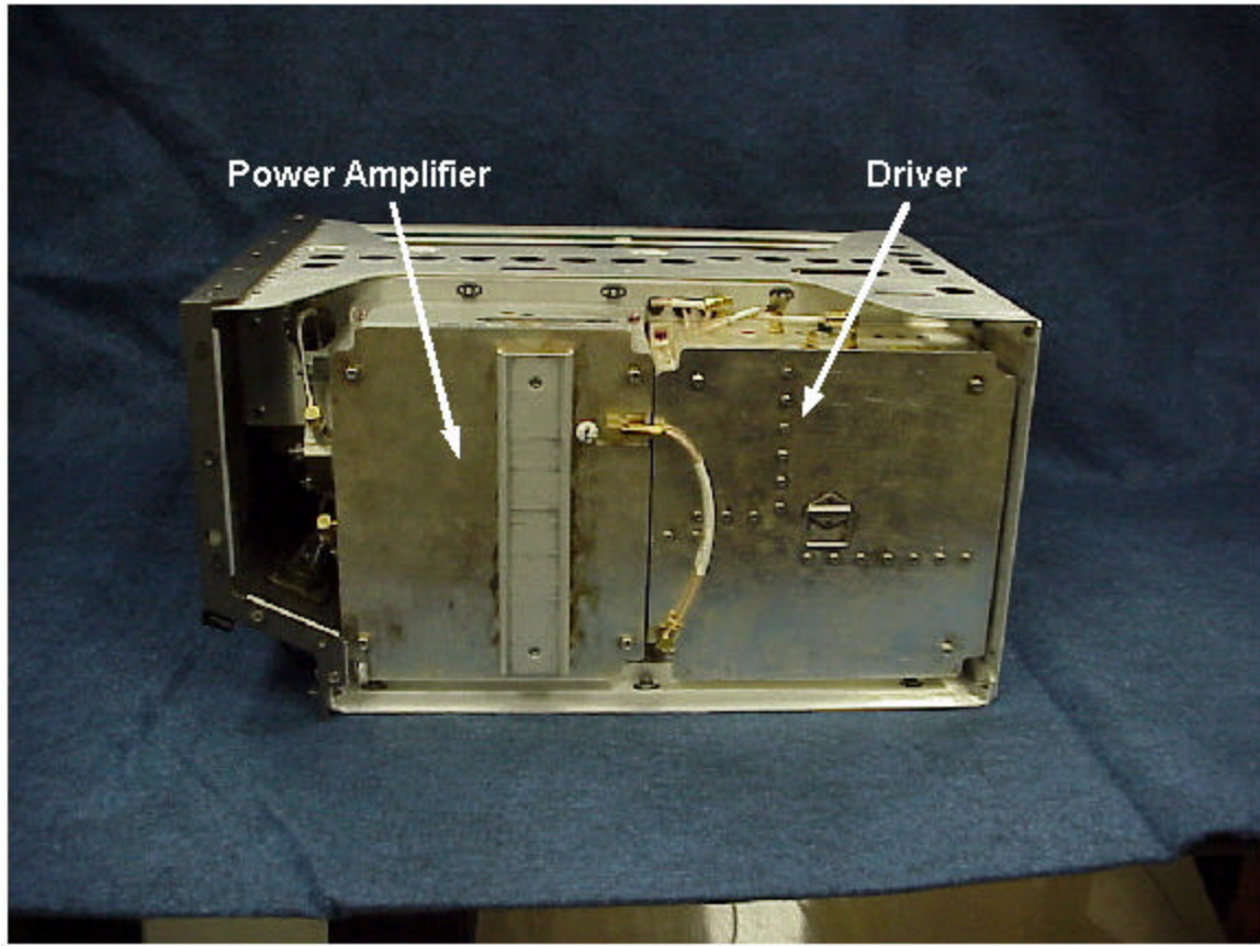
Figure 7-4. Right Side
