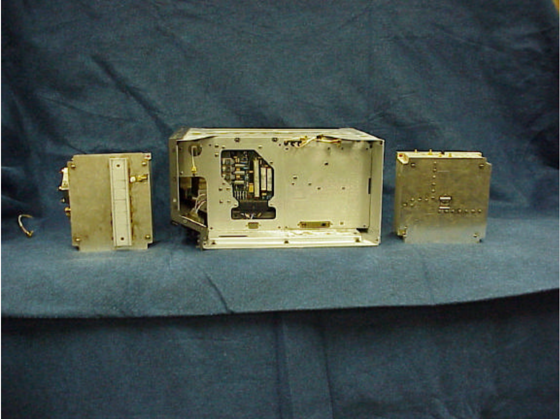
Figure 7-8. Right Modules Removed
