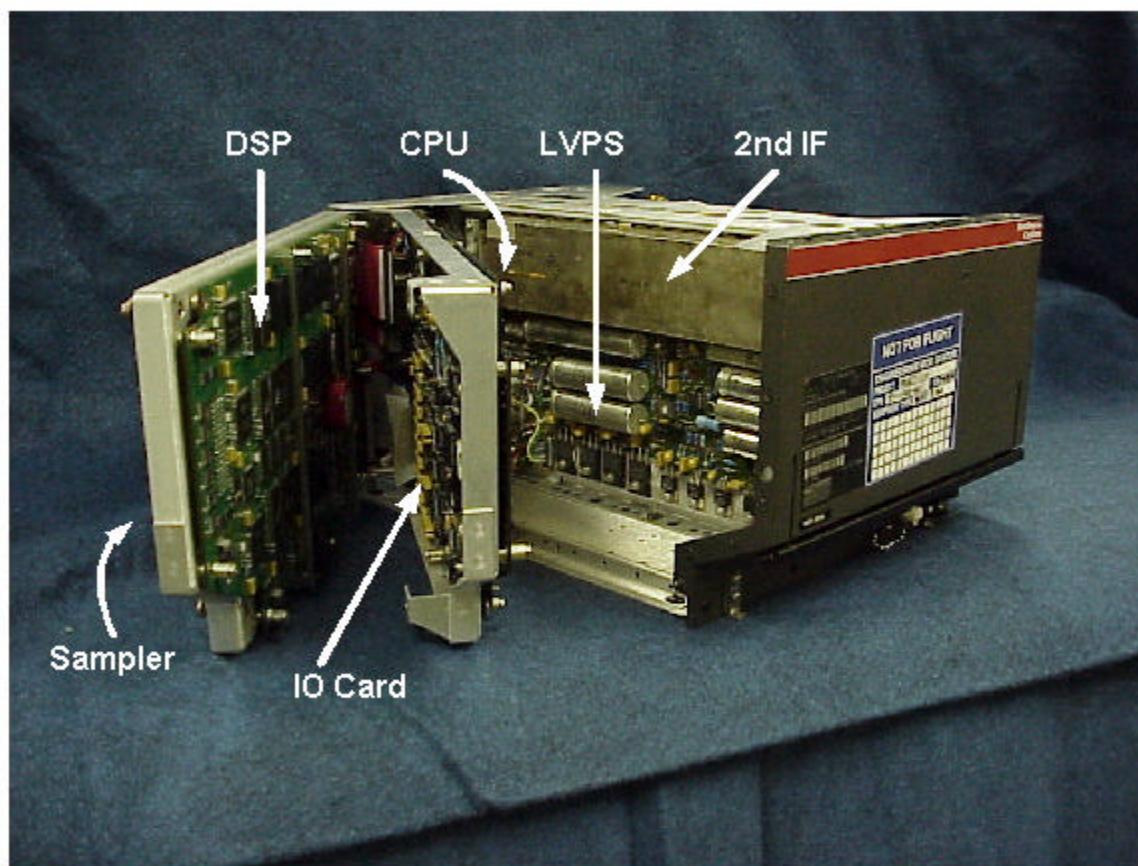
Figure 7-7. Left Open
