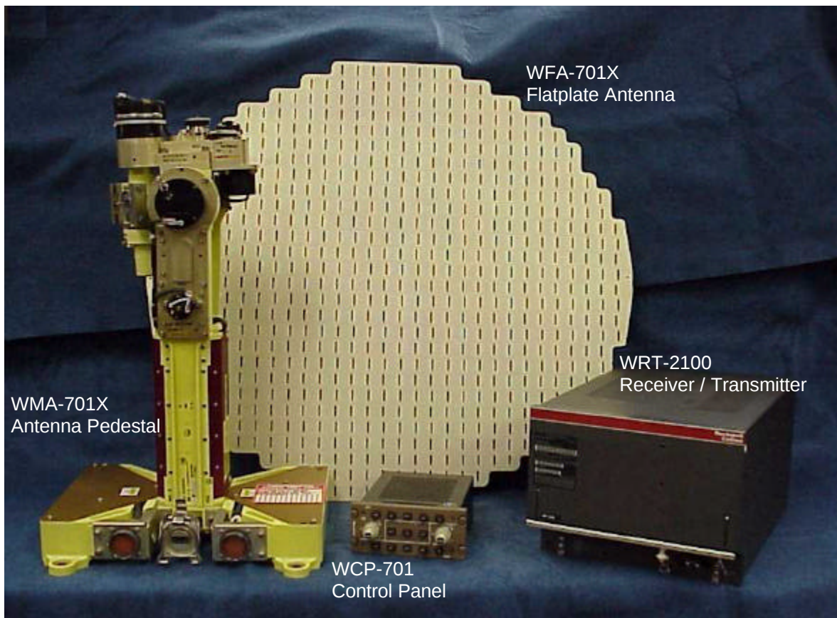
Figure 7-1. WXR-2100 Family
