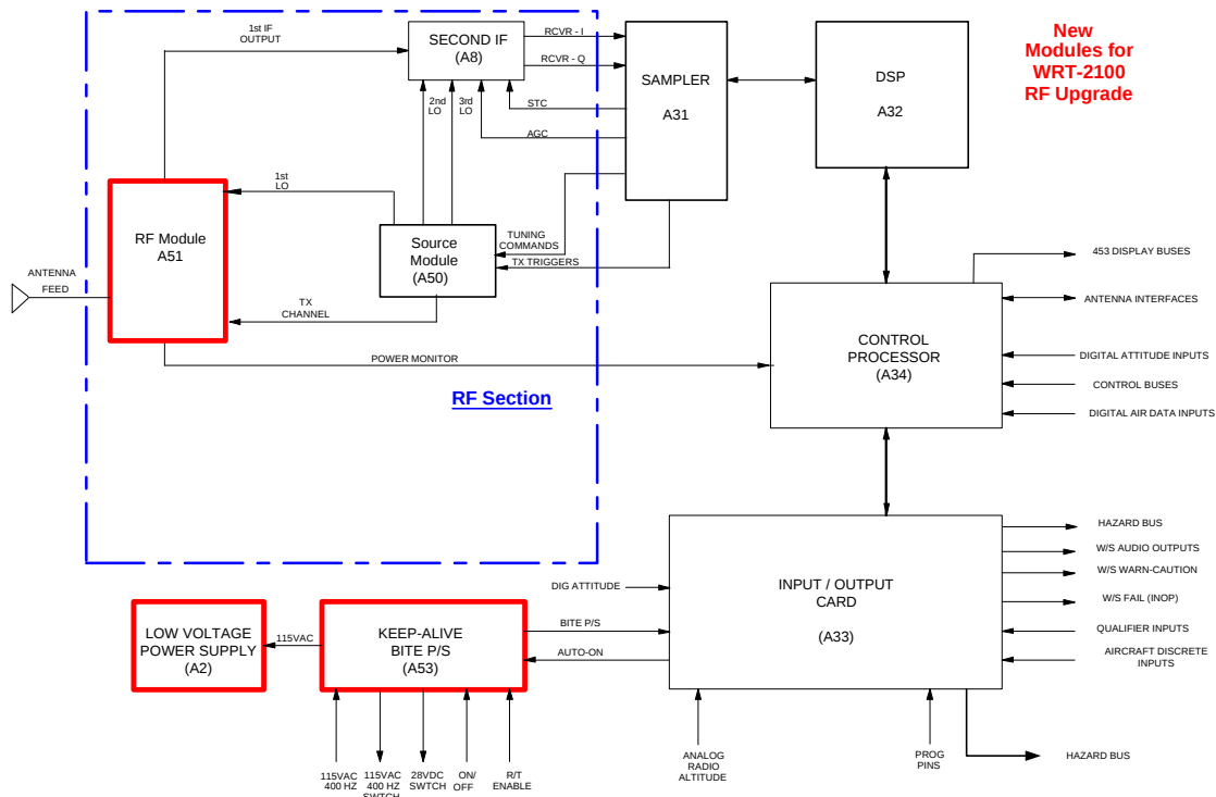
Figure L-4. WRT-2100 Receiver-Transmitter Simplified Block Diagram
