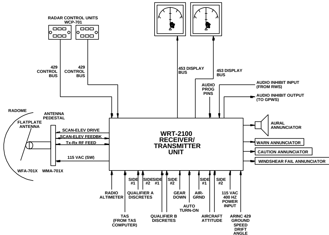
Figure L-2. Typical WXR-2100 Aircraft Installation
