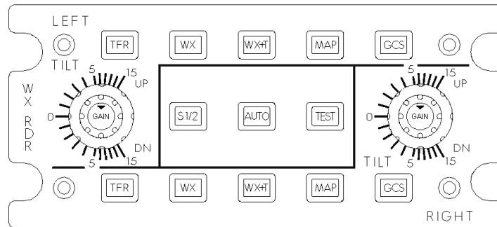
Figure L-3. WCP-702 Dual Control Panel
