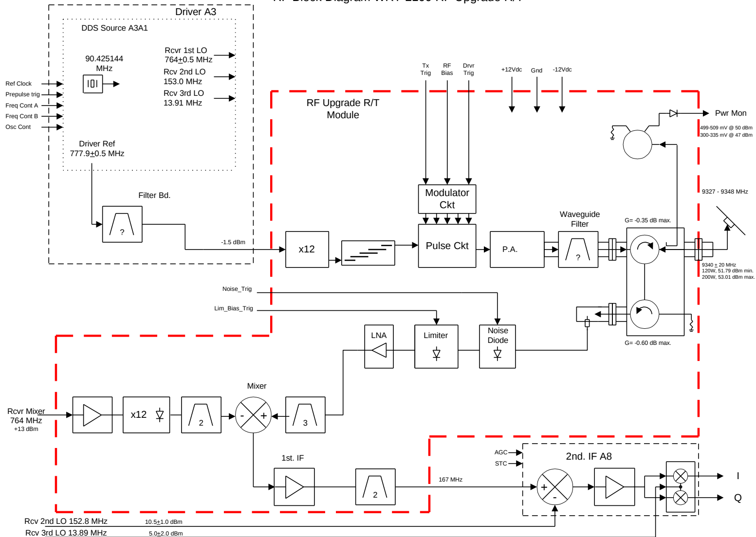
Figure L-5. WRT-2100 RF Section Block Diagram
