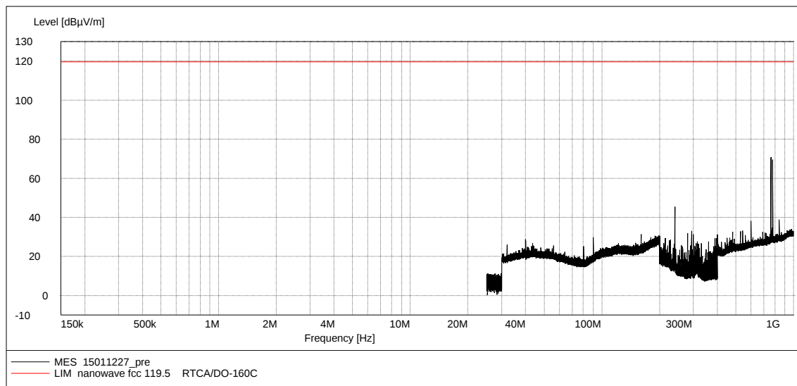
Figure F-69. Radiated Spurious Emissions, Normal Mode, 25 MHz to 1 GHz, (Horizontal Polarization),
