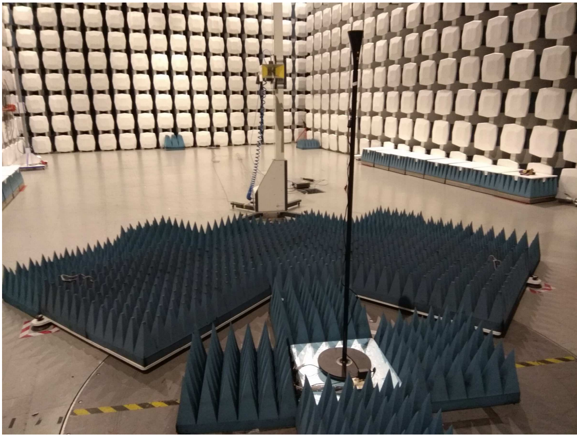
Radiated Emissions 1 GHz – 18 GHz
