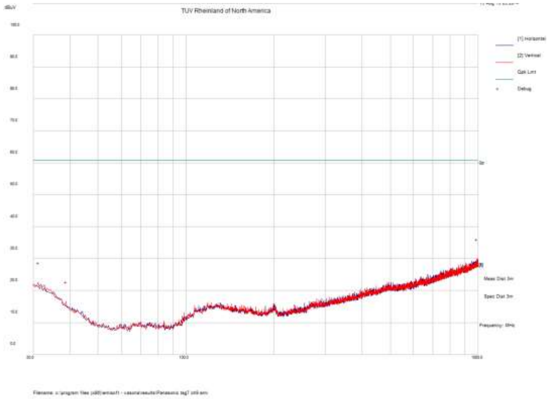
Figure 23: 30-1000 MHz, 434.568 MHz
