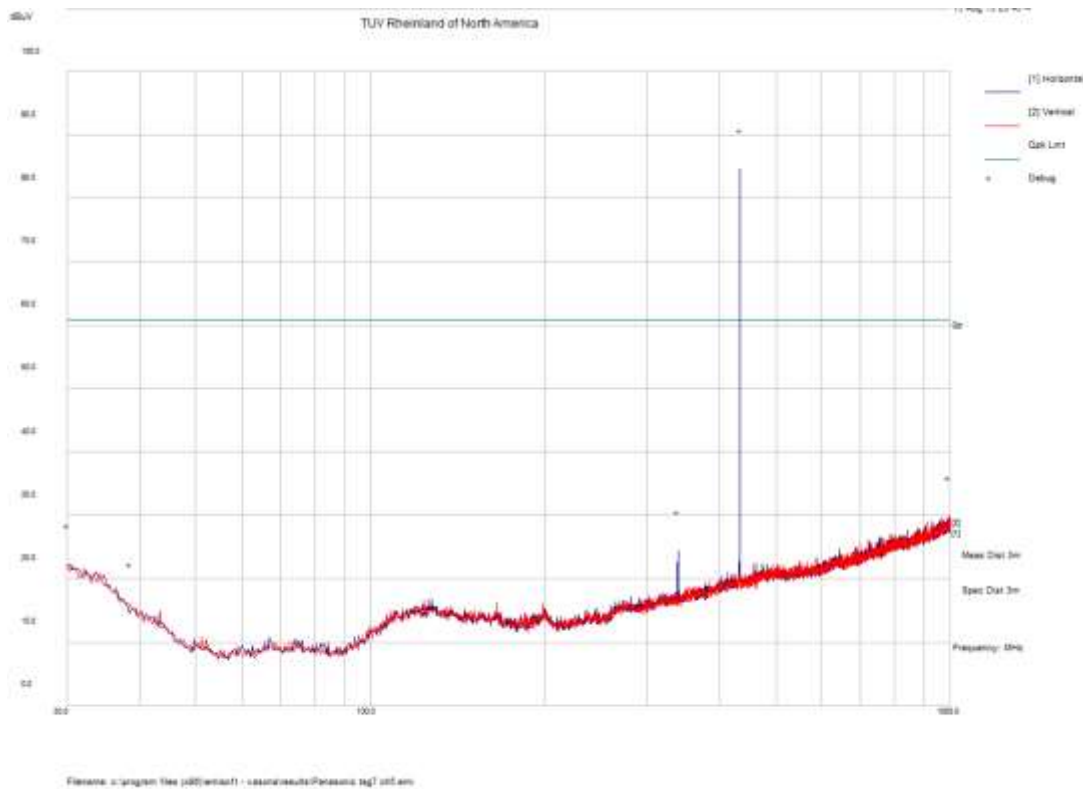
Figure 21: 30-1000 MHz, 433.704 MHz
