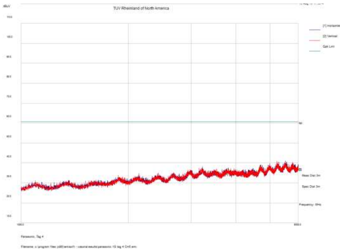
Figure 22: 1-6GHz, 433.704 MHz
