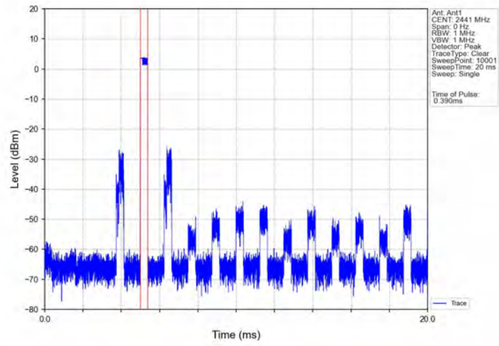
Dwell_Time_(Hopping)_NVNT_ANT1_2-DH1_2441_Accumulated
