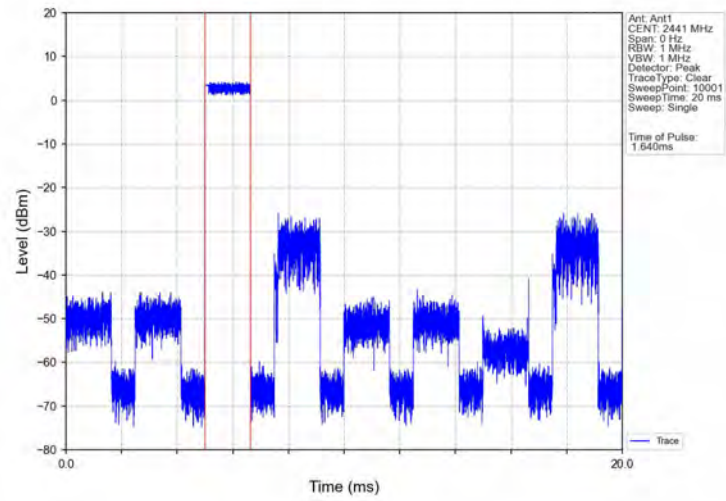
Dwell_Time_(Hopping)_NVNT_ANT1_3-DH3_2441_Accumulated
