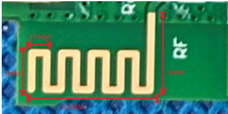
Antenna Photo & Length (mm)
