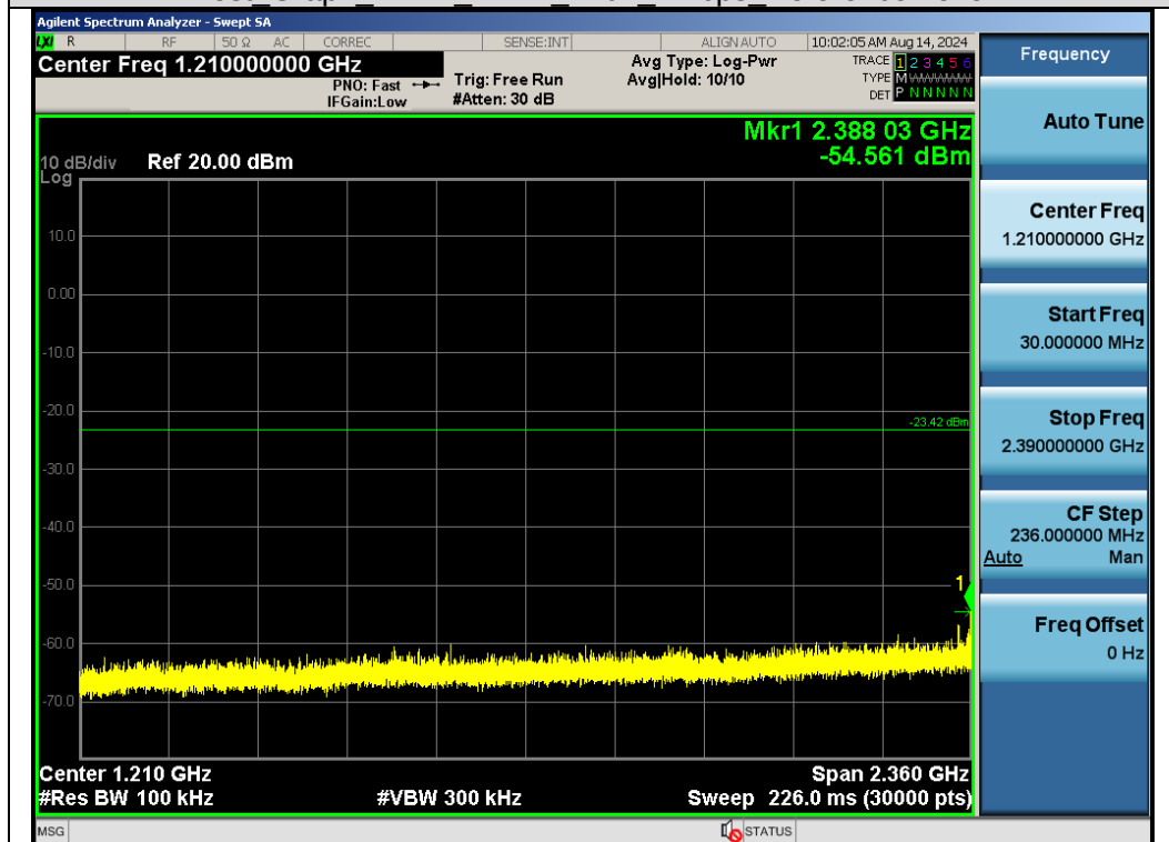
Test Graph LE1M ANT1 2402 1Mbps Lower Band Emissions
