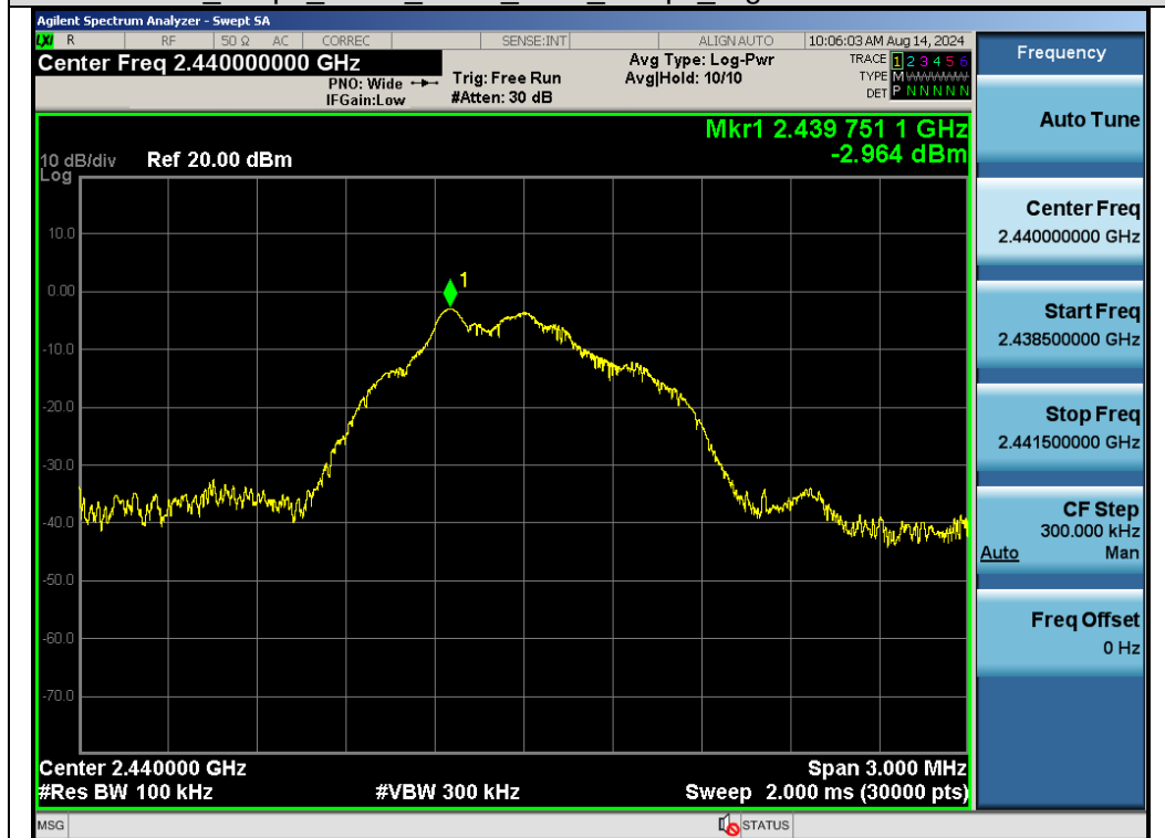
Test_Graph_LE1M_ANT1_2440_1Mbps_Reference Level
