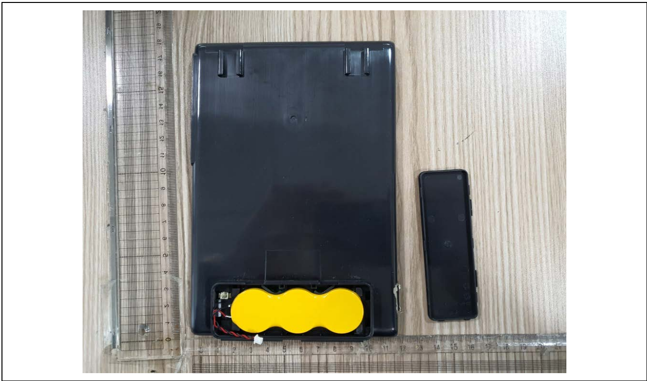
Battery Position
