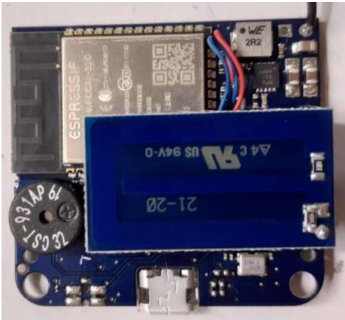
Assembled Boards
