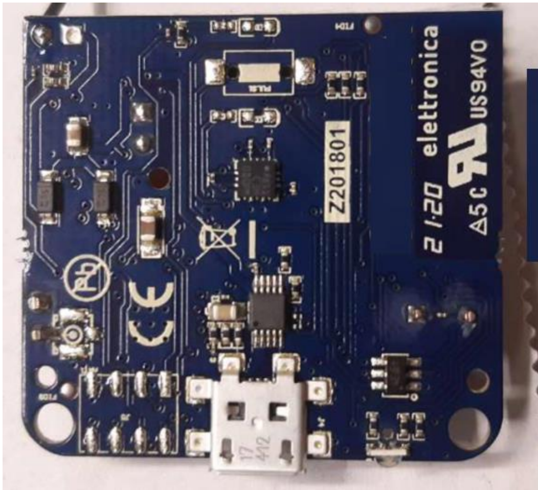
Main PCB
