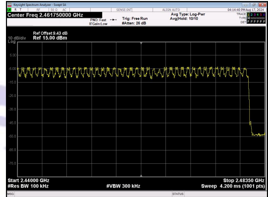
High End Spectrum Channel Hopping Plot
