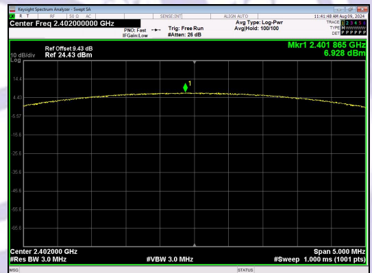
Peak Output Power
