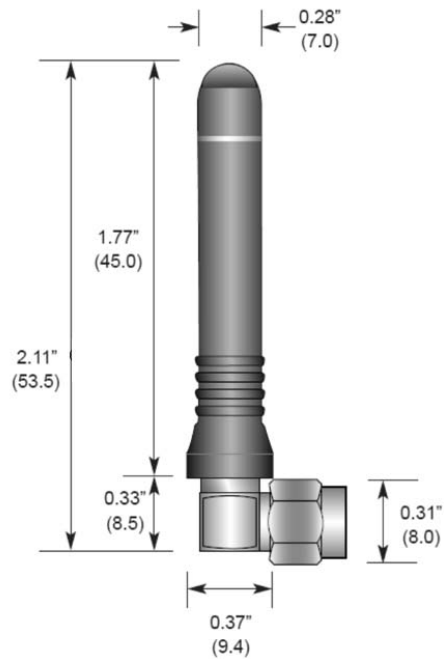
Figure 2: Antenna Dimensions
