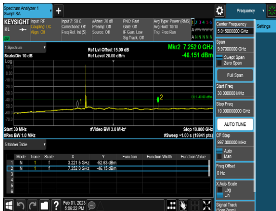
SCC_20M_3634.9MHz_Q16_1RB_CSE3
