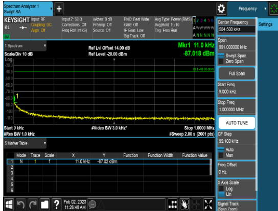
SCC_20M_3634.9MHz_Q64_1RB_CSE1
