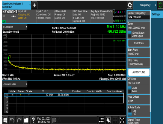
SCC_20M_3634.9MHz_Q16_FULLLRB_CSE1
