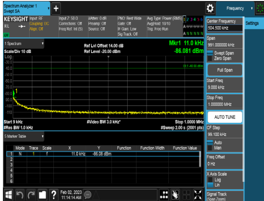
SCC_20M_3579.8MHz_Q64_FULLLRB_CSE1
