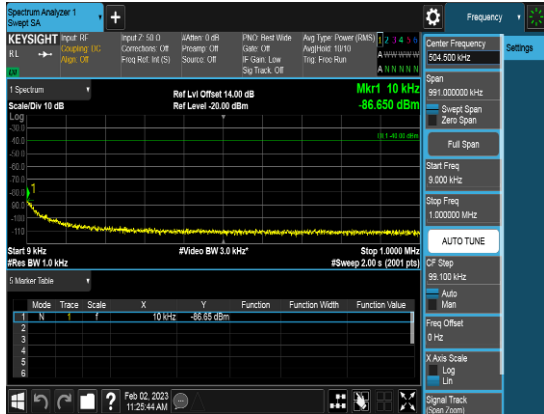
SCC_20M_3634.9MHz_Q16_1RB_CSE1
