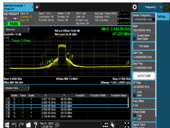
SCC_20M_3579.8MHz_Q64_FULLLRB_CSEpart9 6
