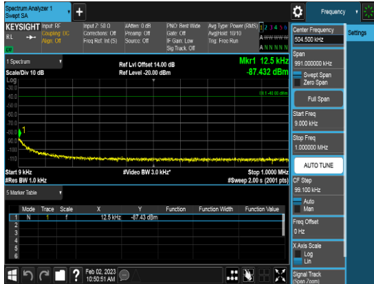
PCC_20M_3670.2MHz_QPSK_FULLLRB_CSE1
