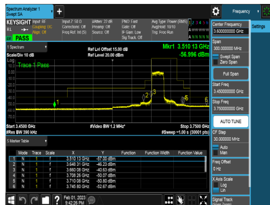
PCC_20M_3670.2MHz_QPSK_FULLLRB_CSEpar t96
