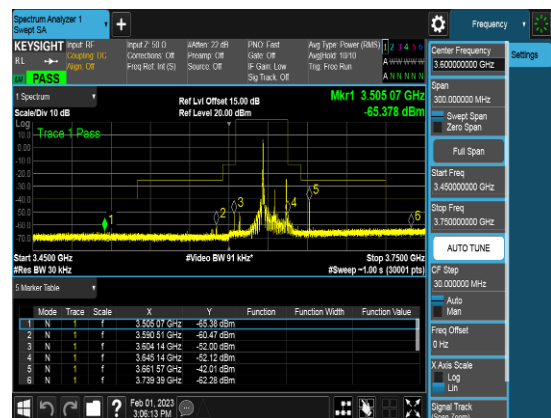
SCC_20M_3634.9MHz_Q64_1RB_CSEpart96
