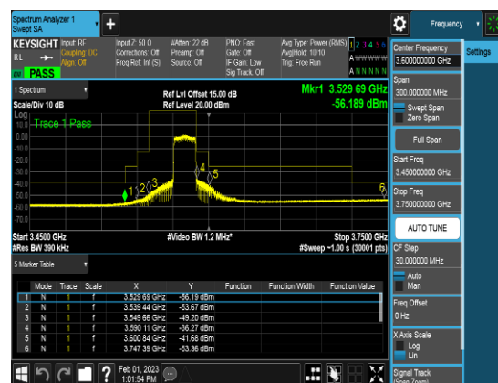
SCC_20M_3579.8MHz_QPSK_FULLLRB_CSEpar t96
