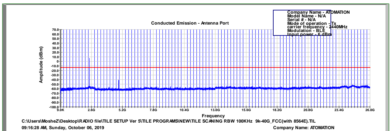
Figure 35 2440.0 MHz, BLE
