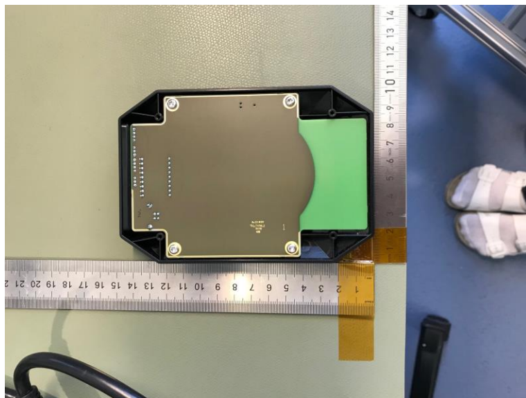
Figure 2: Top half Anchor viewed from Bottom
