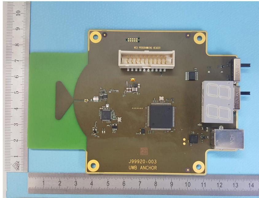
Figure 3: PCB removed from top half of anchor, viewed from top
