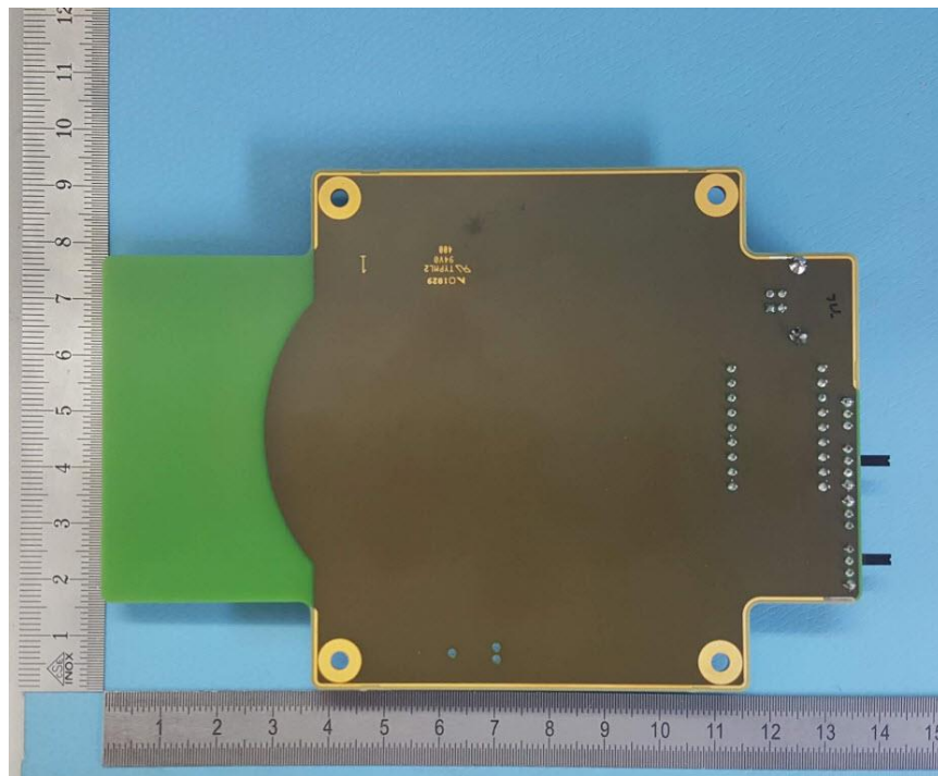
Figure 4: PCB removed from top half of anchor, viewed from bottom
