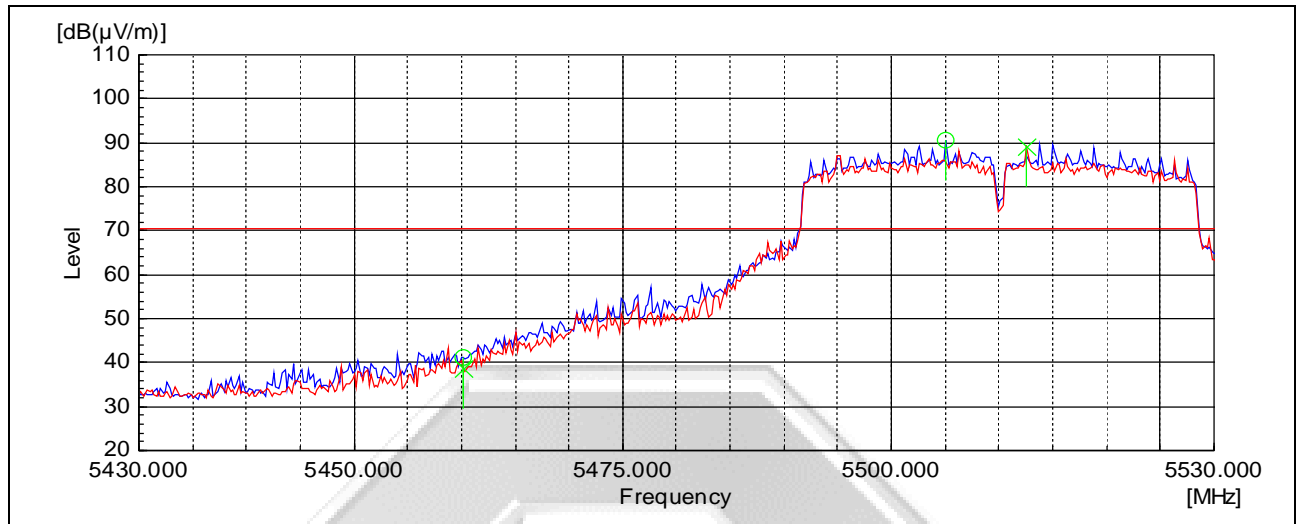
Plot 16 – Lower Band Edge at 5.46GHz
