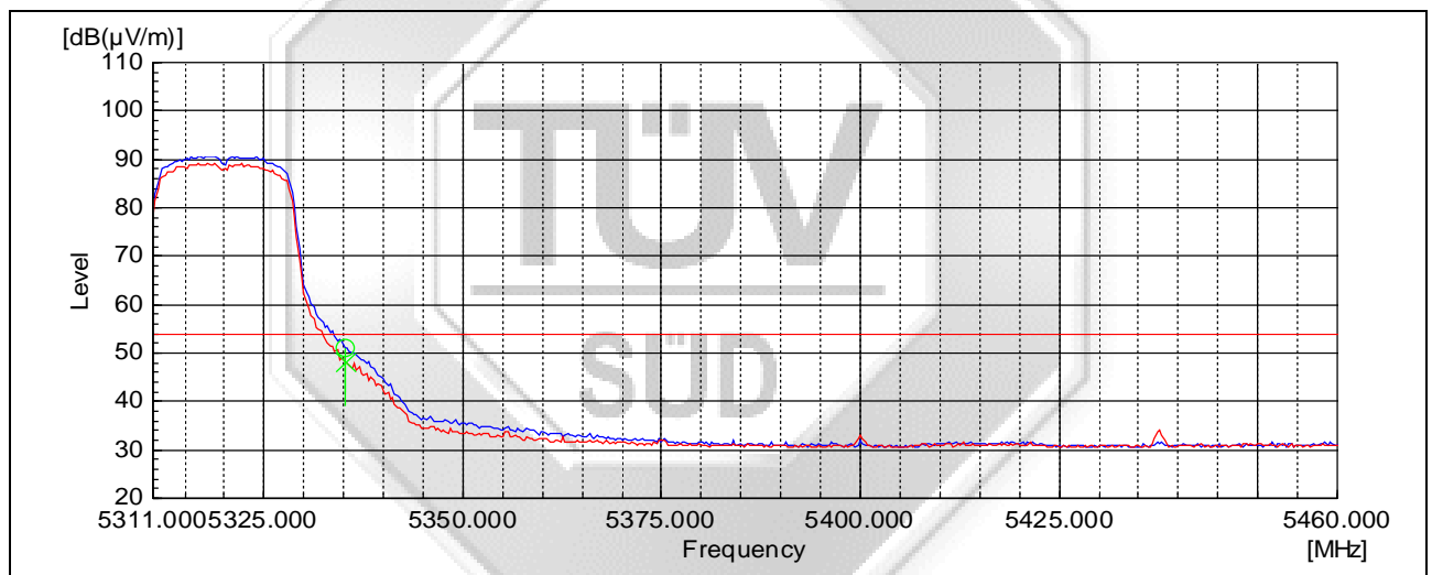
Plot 6 – Average Plot at Upper Band Edge at 5.35GHz
