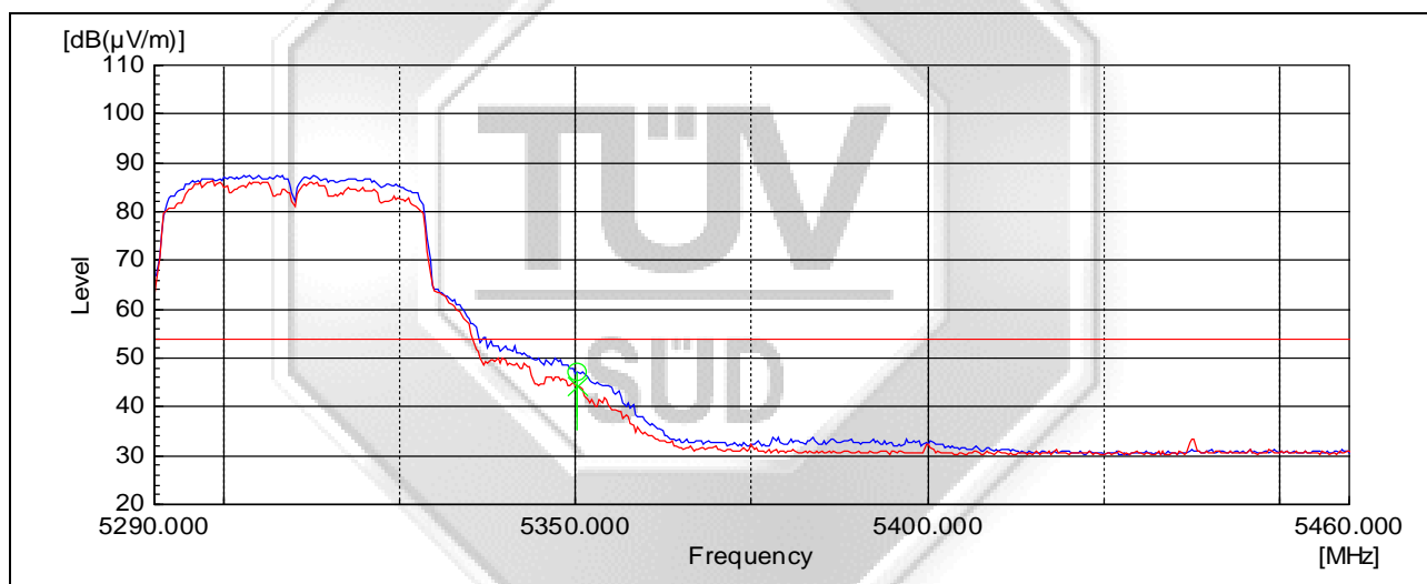
Plot 15 – Average Plot at Upper Band Edge at 5.35GHz
