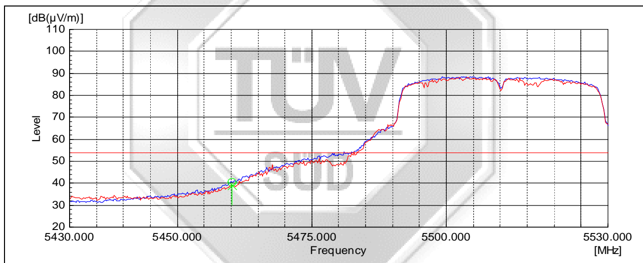
Plot 18 – Average Plot at Lower Band Edge at 5.46GHz
