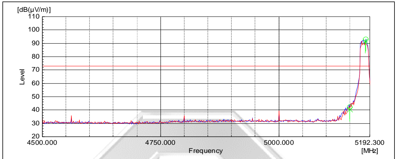
Plot 1 – Lower Band Edge at 5.15GHz
