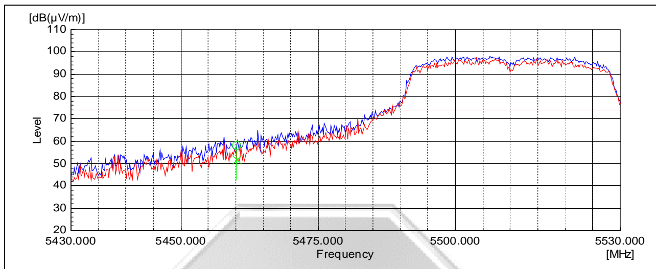
Plot 17 – Peak Plot at Lower Band Edge at 5.46GHz
