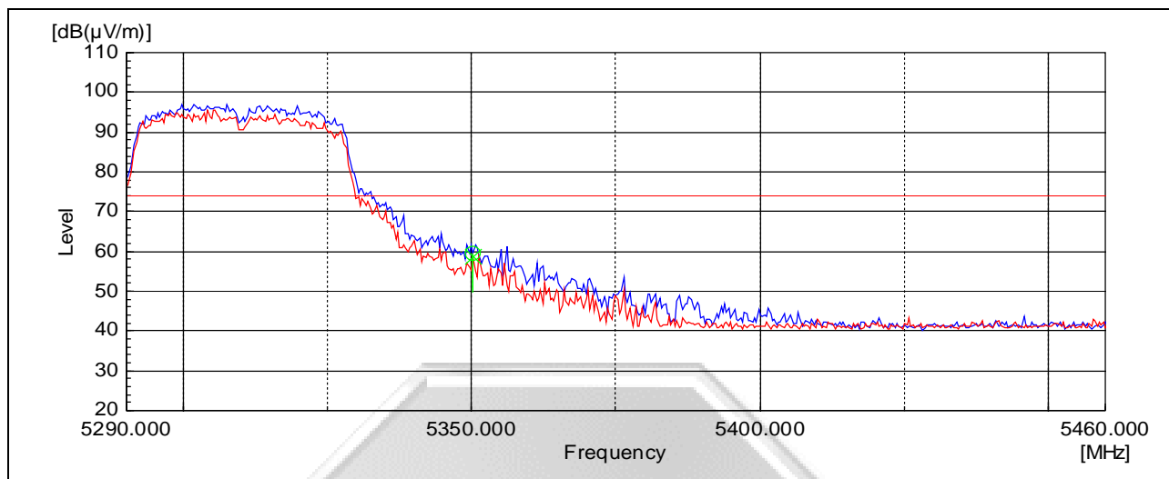
Plot 14 – Peak Plot at Upper Band Edge at 5.35GHz
