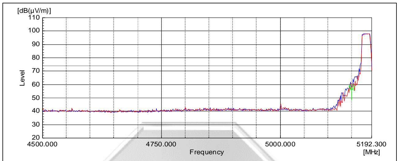
Plot 3 – Peak Plot at Lower Band Edge at 5.15GHz
