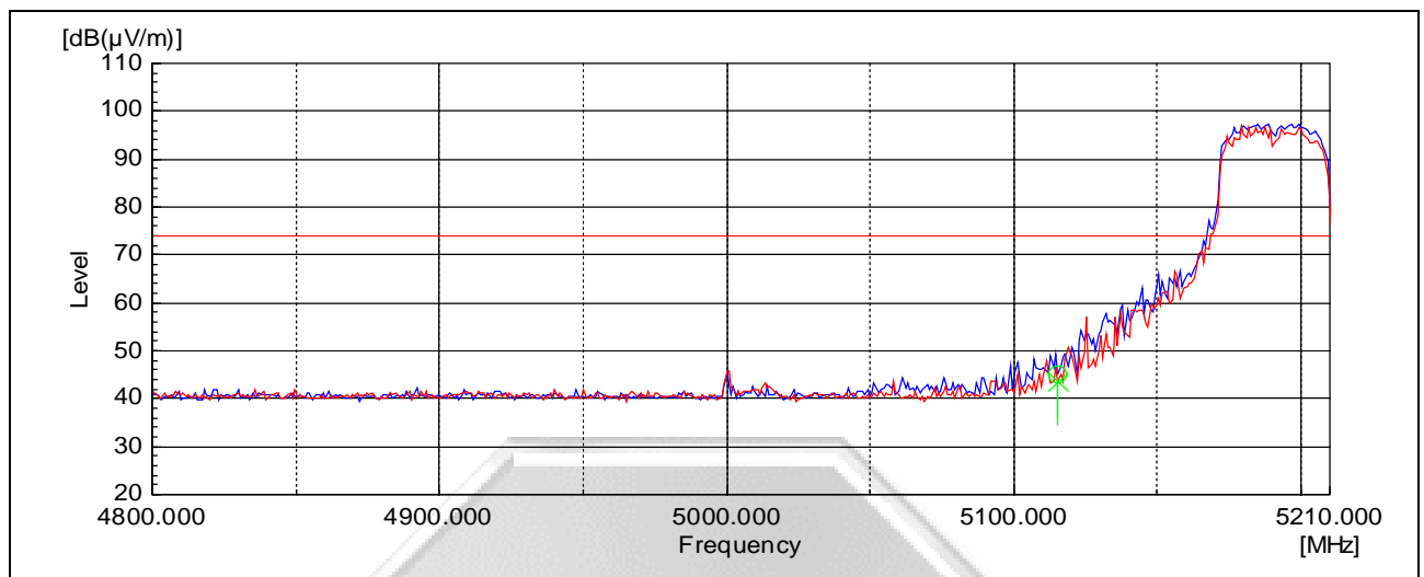
Plot 12 – Peak Plot at Lower Band Edge at 5.15GHz
