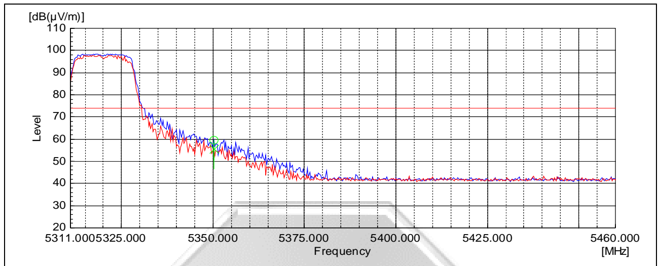
Plot 5 – Peak Plot at Upper Band Edge at 5.35GHz
