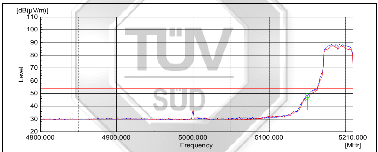
Plot 13 – Average Plot at Lower Band Edge at 5.15GHz
