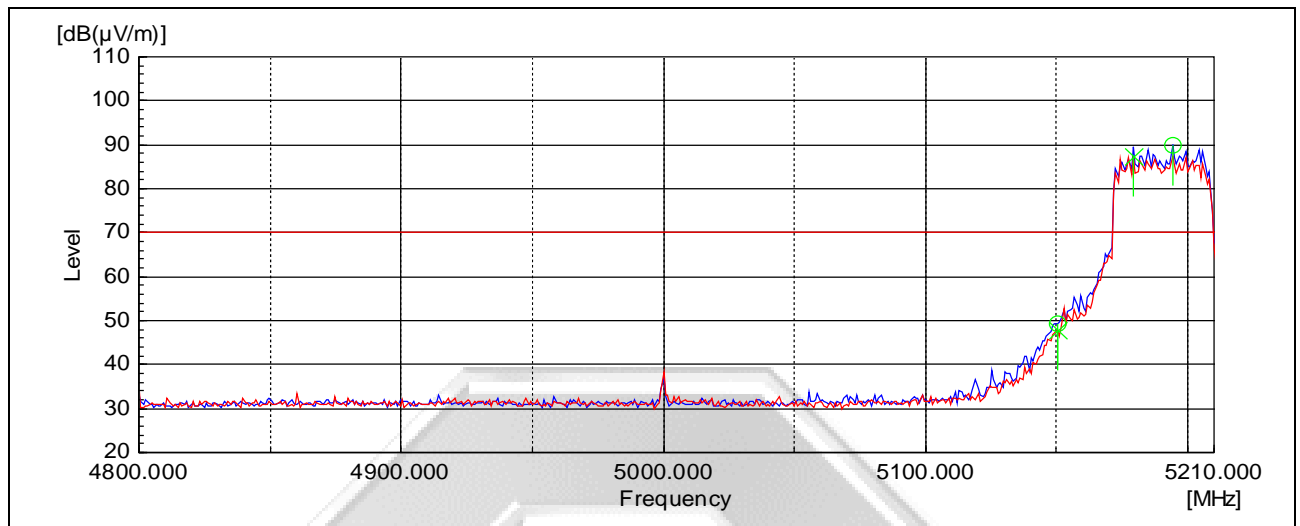
Plot 10 – Lower Band Edge at 5.15GHz
