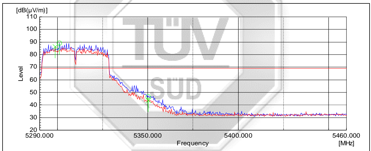
Plot 11 – Upper Band Edge at 5.35GHz
