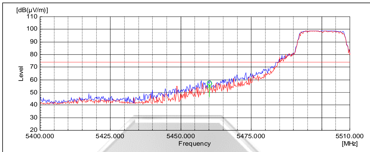
Plot 8 – Peak Plot at Lower Band Edge at 5.46GHz
