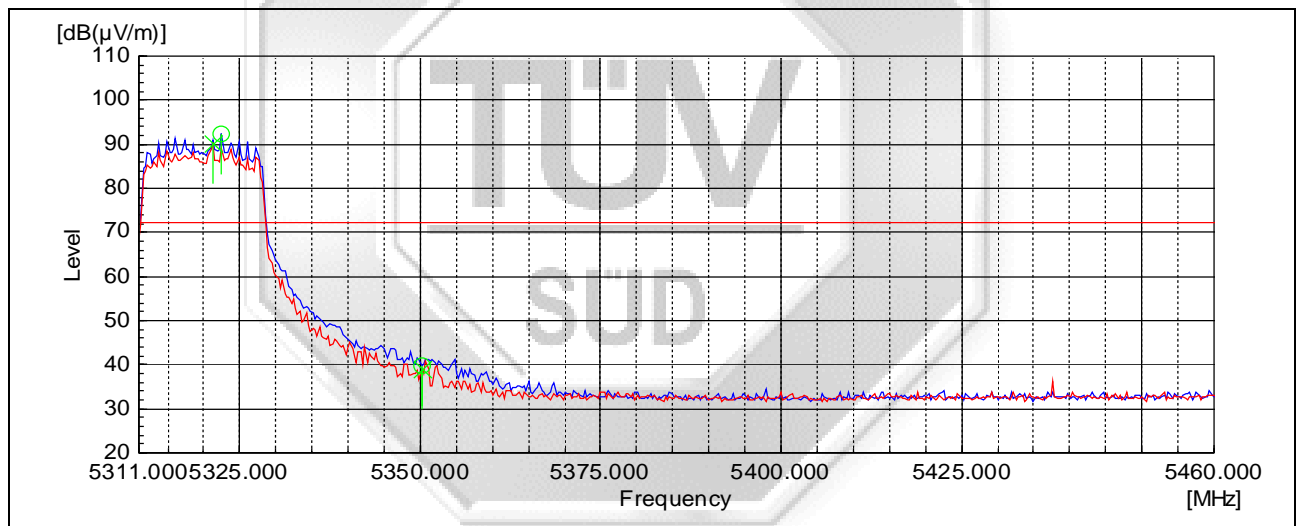
Plot 2 – Upper Band Edge at 5.35GHz
