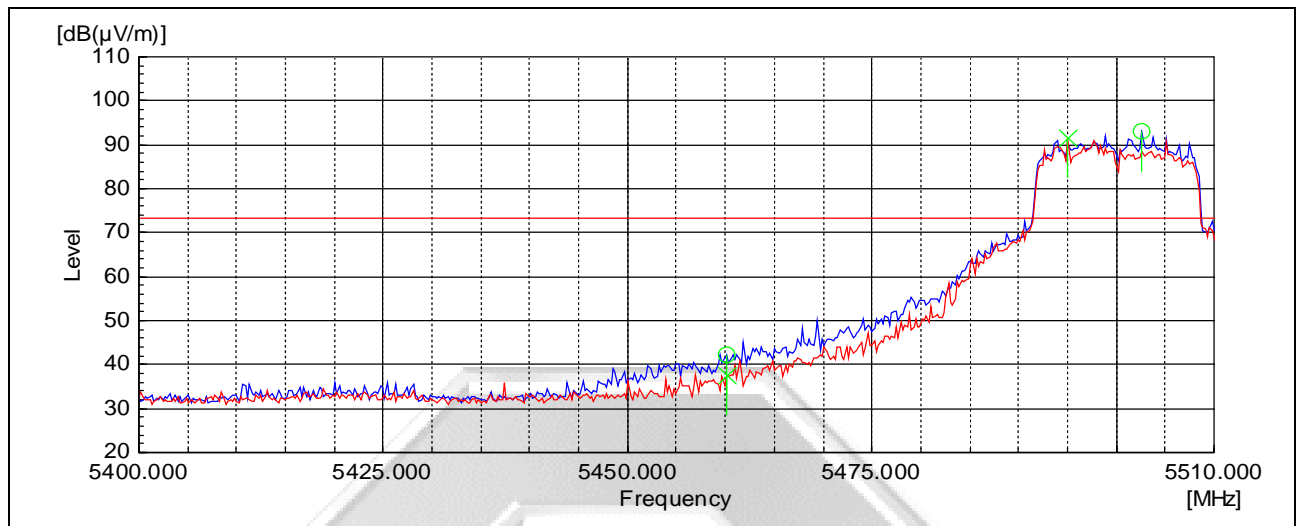
Plot 7 – Lower Band Edge at 5.46GHz
