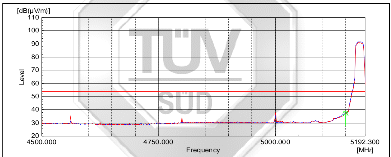
Plot 4 – Average Plot at Lower Band Edge at 5.15GHz
