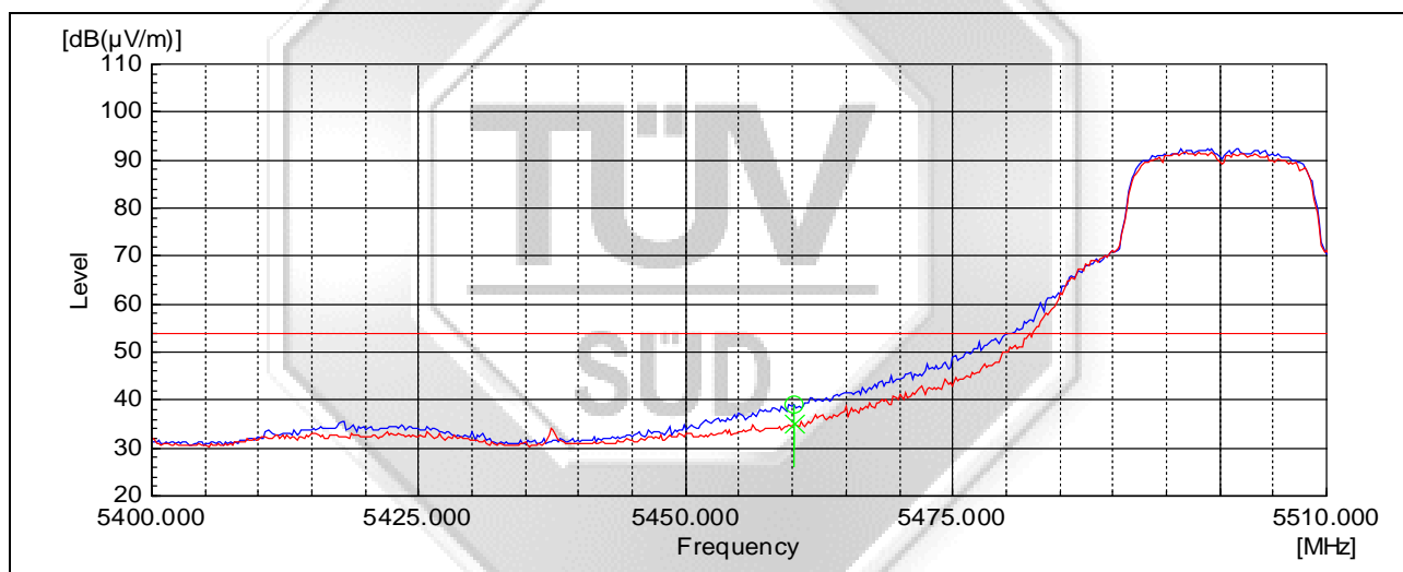
Plot 9 – Average Plot at Lower Band Edge at 5.46GHz
