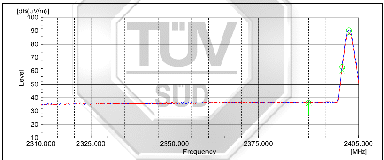
Plot 4 – Average Plot at Lower Band Edge at 2.4000GHz
