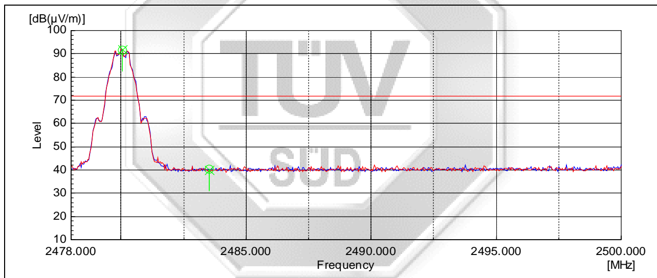
Plot 2 – Upper Band Edge at 2.4835GHz
