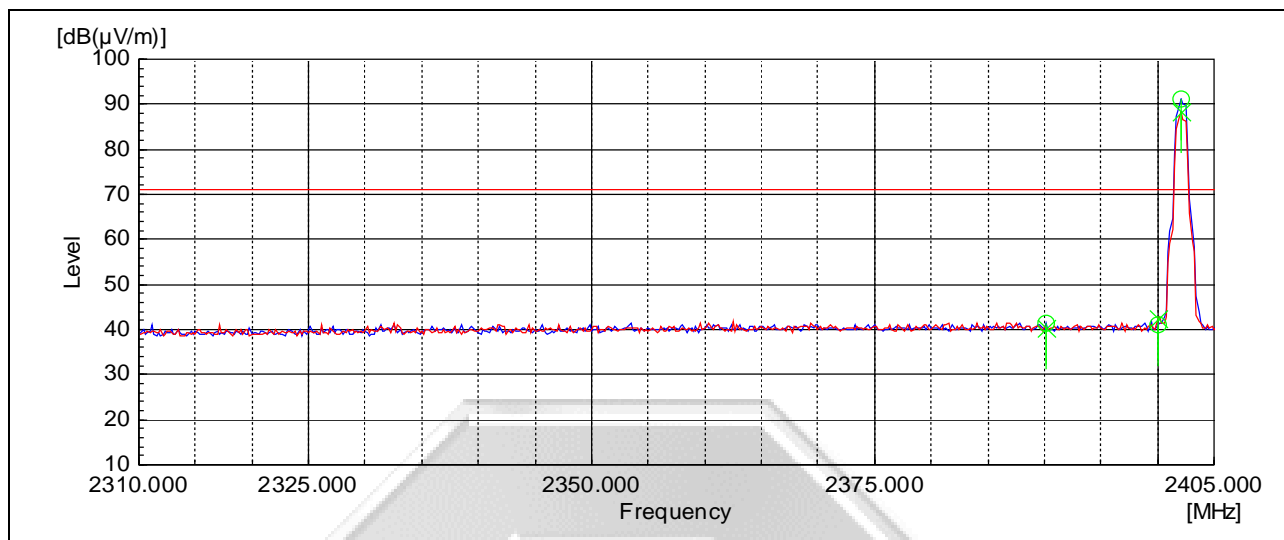
Plot 1– Lower Band Edge at 2.4000GHz
