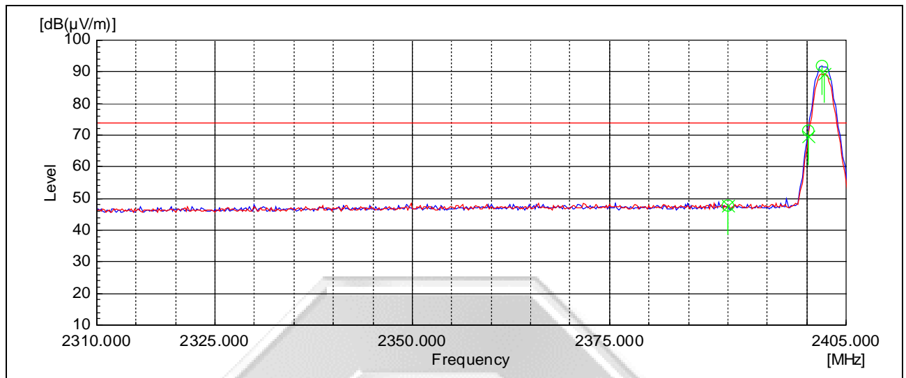
Plot 3 – Peak Plot at Lower Band Edge at 2.4000GHz
