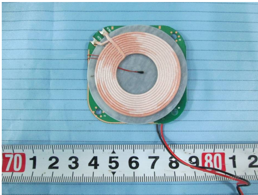
EUT – Charging Coil Board Top View
