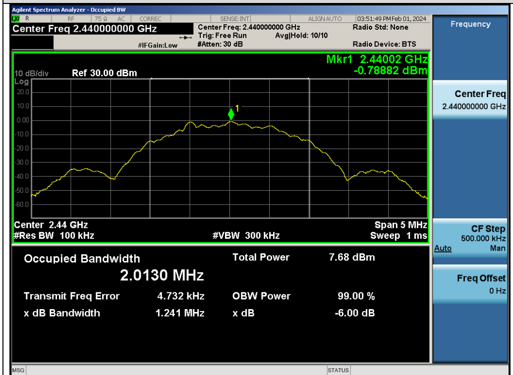
Test_Graph_LE2M_ANT1_2440_2Mbps_DTSBW
