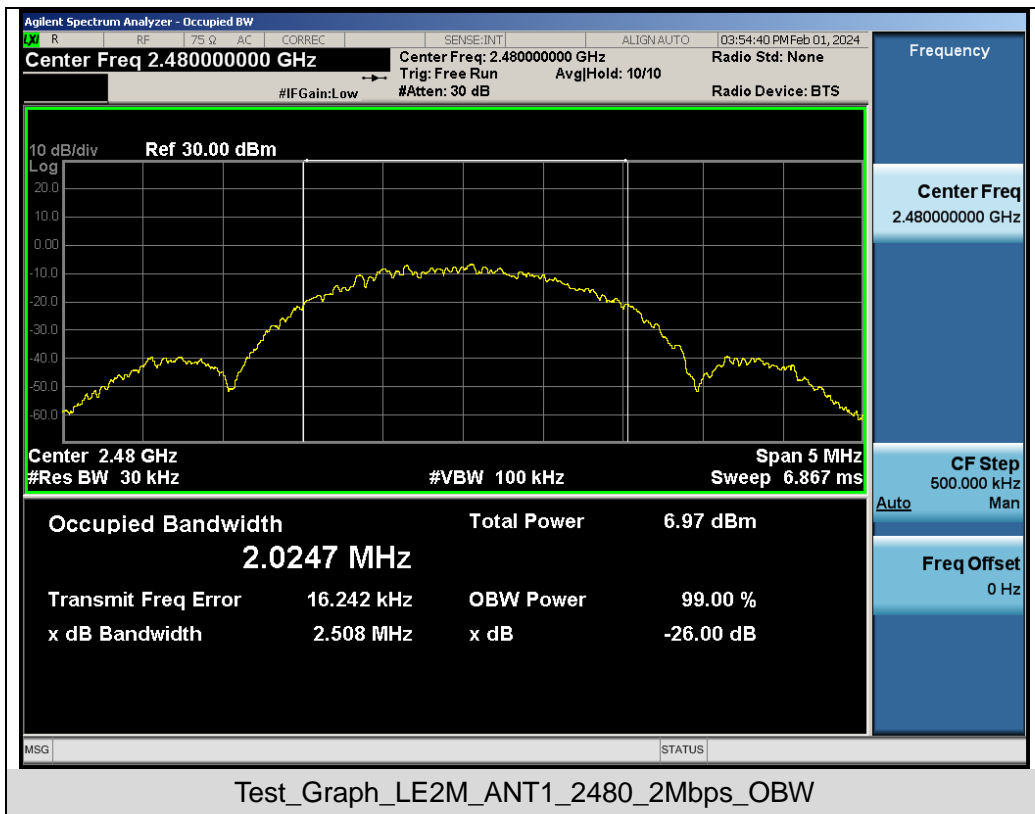
Test_Graph_LE2M_ANT1_2480_2Mbps_OBW
