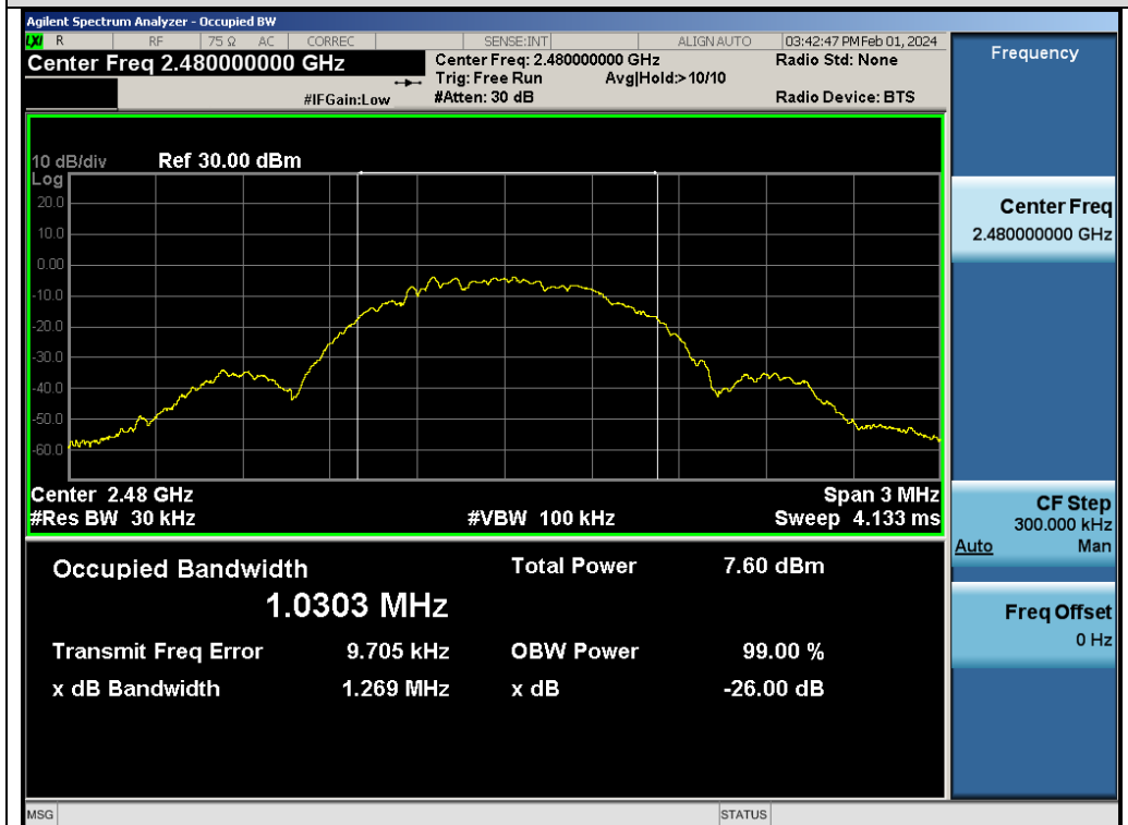
Test_Graph_LE1M_ANT1_2480_1Mbps_OBW
