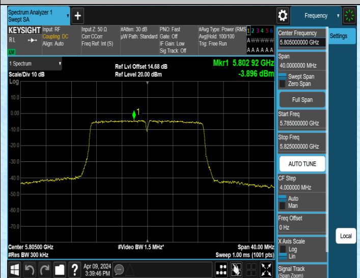
11AC20MIMO-Ant2-5805-PASS
