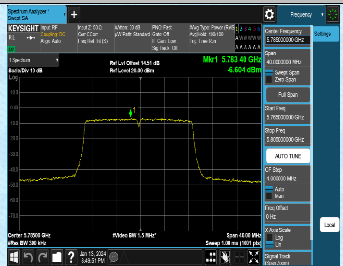
11AC20MIMO-Ant2-5785-PASS
