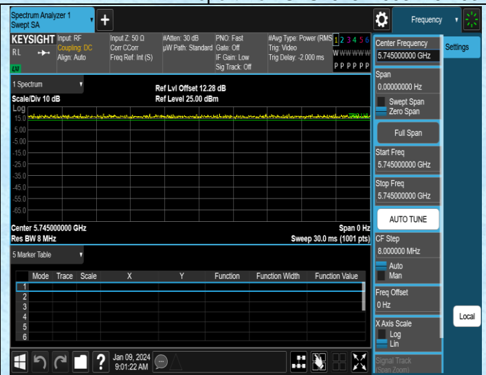
NTNV-11AC20SISO-Ant4-5745
