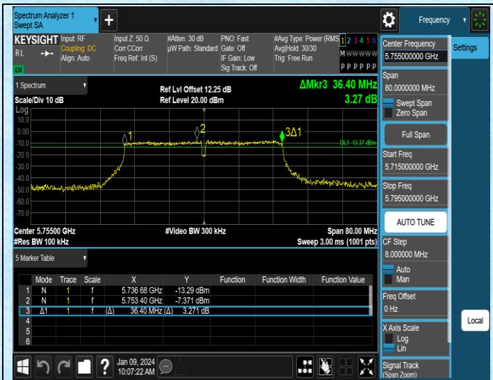
11AC40MIMO-Ant3-5755-PASS
