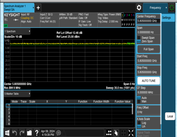
NTNV-11N20SISO-Ant4-5805
