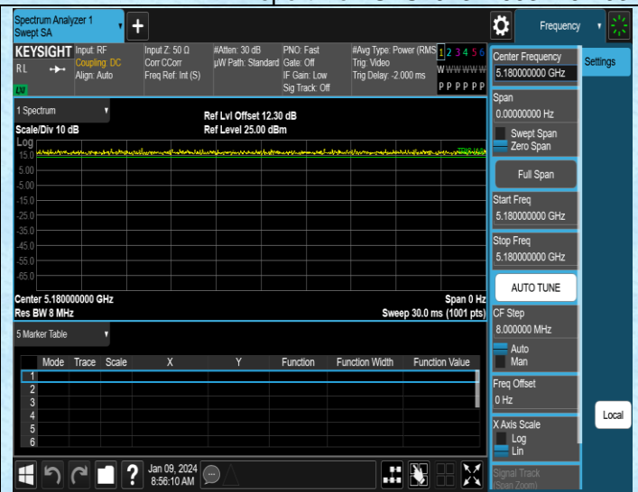
NTNV-11AC20SISO-Ant4-5180
