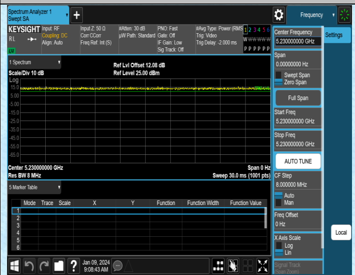
NTNV-11AC40SISO-Ant4-5230
