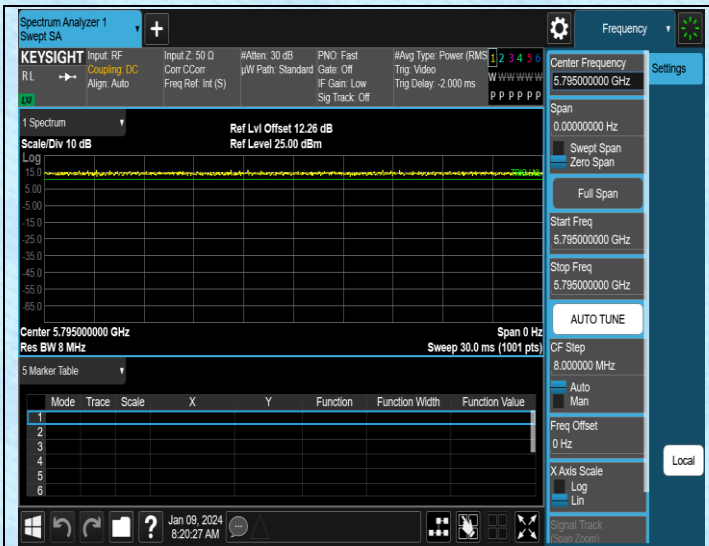
NTNV-11AC40SISO-Ant3-5795
