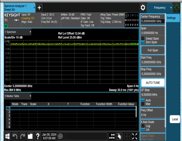
NTNV-11AC20SISO-Ant4-5200
