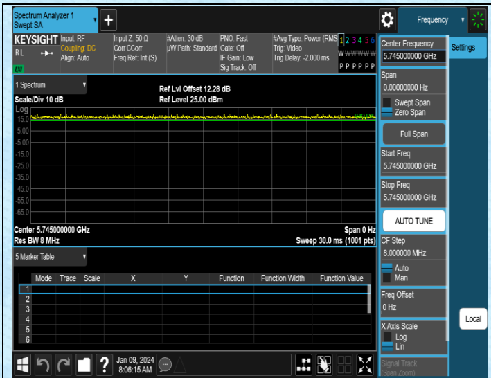
NTNV-11AC20SISO-Ant3-5745
