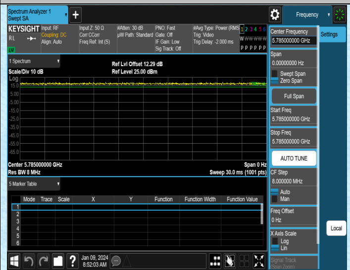
NTNV-11N20SISO-Ant4-5785
