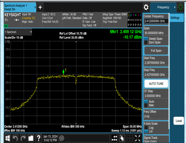
11N20MIMO-Ant2-2412-0~Reference-PASS
