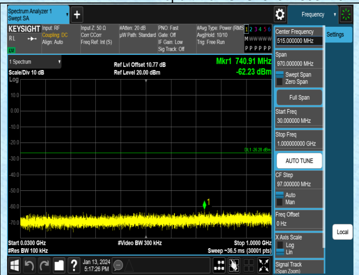
11N20SISO-Ant1-2437-30~1000-PASS
