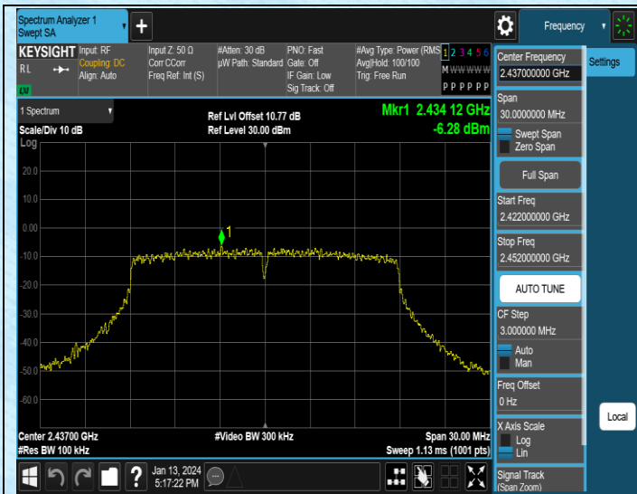
11N20SISO-Ant1-2437-0~Reference-PASS
