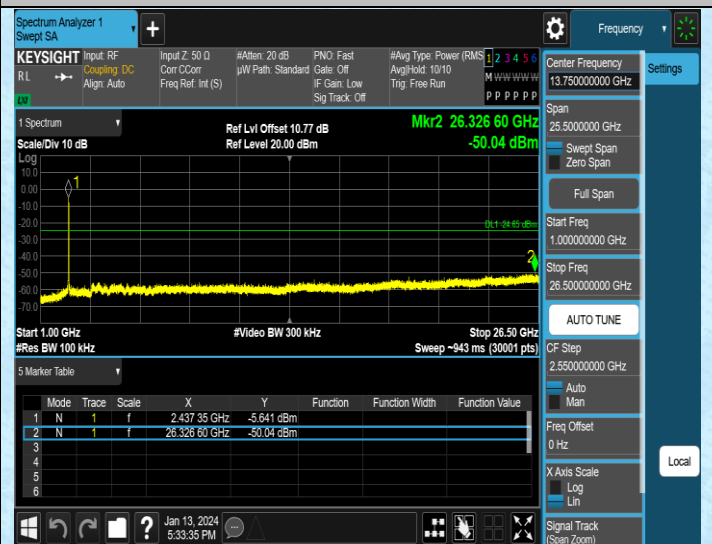
11N20SISO-Ant2-2437-1000~26500-PASS
