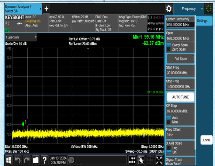
11N20MIMO-Ant1-2412-30~1000-PASS
