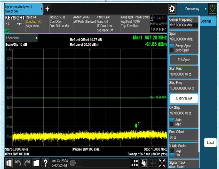
11N20MIMO-Ant1-2437-30~1000-PASS
