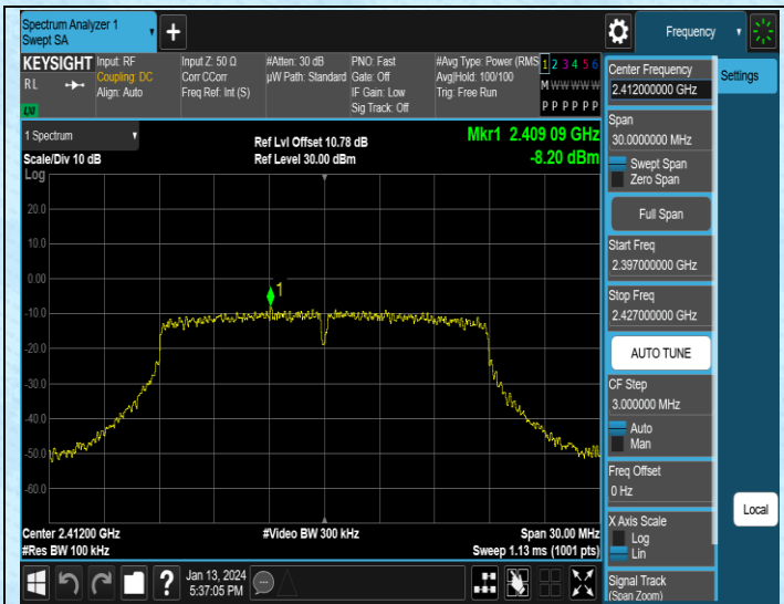
11N20MIMO-Ant1-2412-0~Reference-PASS
