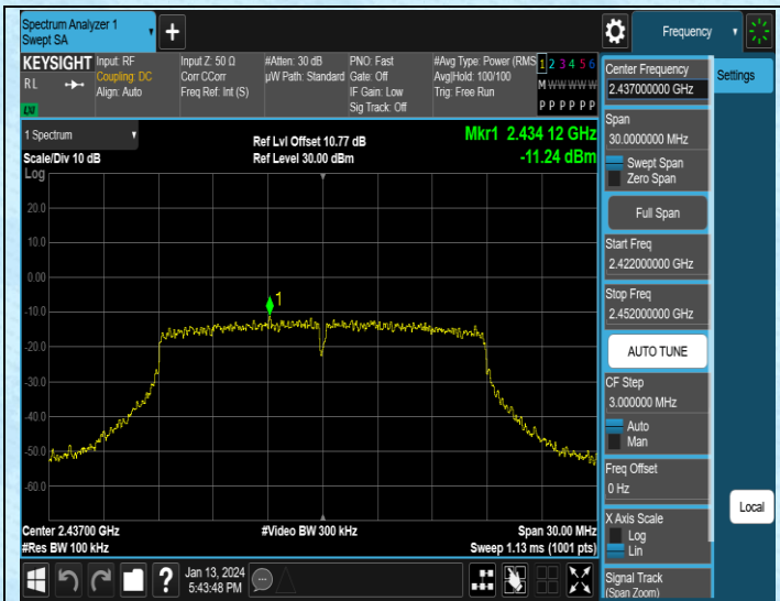
11N20MIMO-Ant1-2437-0~Reference-PASS
