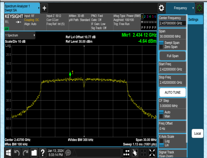
11N20SISO-Ant2-2437-0~Reference-PASS
