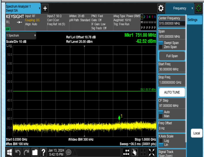
11N20MIMO-Ant2-2412-30~1000-PASS
