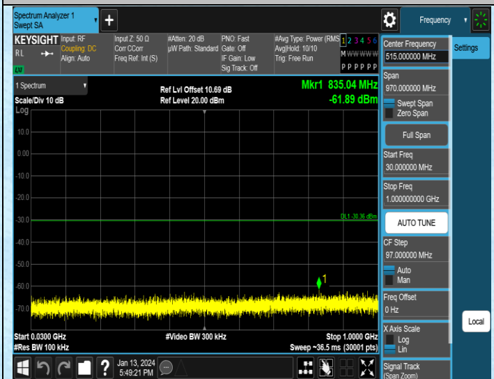
11N20MIMO-Ant2-2462-30~1000-PASS
