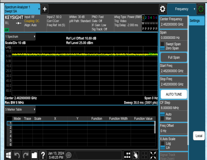
NTNV-11N20MIMO-Ant2-2462
