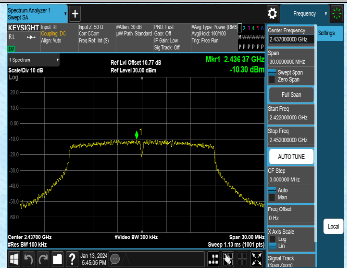
11N20MIMO-Ant2-2437-0~Reference-PASS
