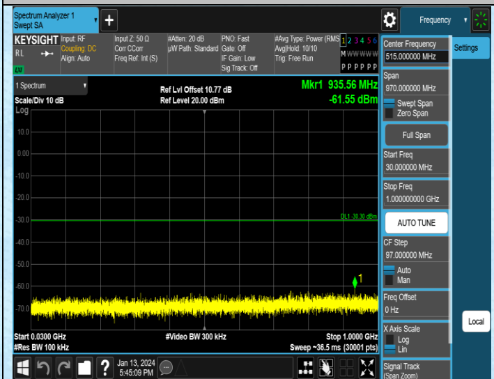
11N20MIMO-Ant2-2437-30~1000-PASS
