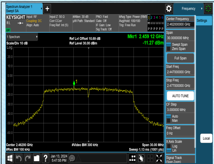
11N20MIMO-Ant1-2462-0~Reference-PASS
