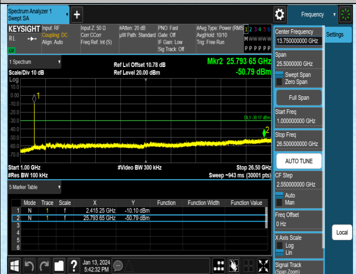
11N20MIMO-Ant2-2412-1000~26500-PASS
