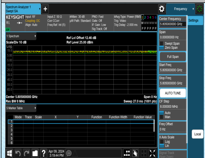
NTNV-11N20SISO-Ant1-5805
