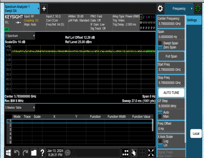
NTNV-11N20MIMO-Ant2-5785
