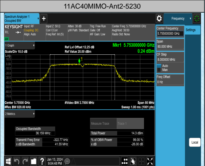
11AC40MIMO-Ant2-5755
