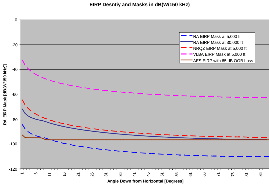
REVISED Figure 5-3 AES EIRP Flux Density Relative to ITU Rec. M.1643
