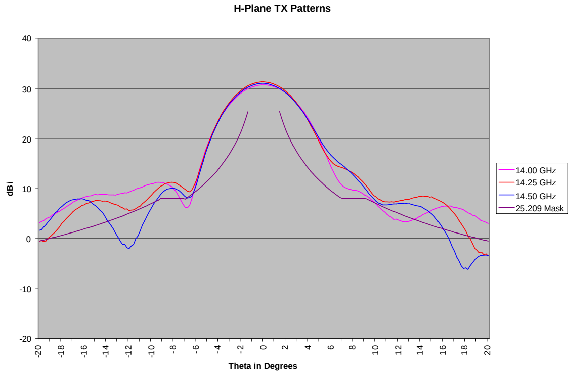
Figure 3-3 Measured Transmit H-Plane Pattern
