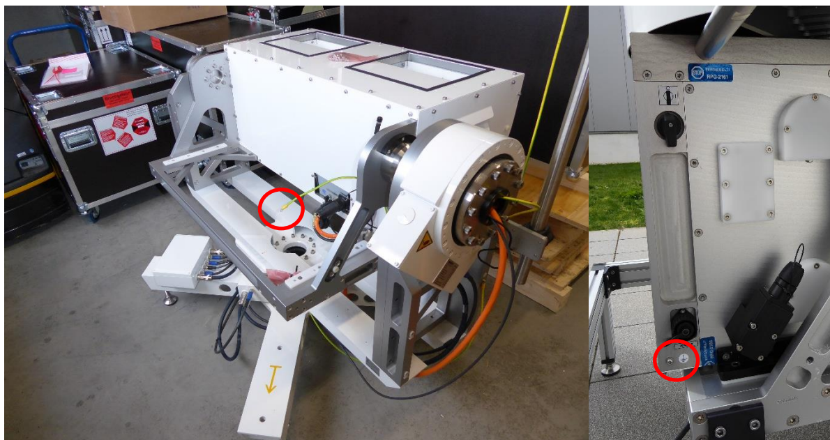
Grounding cable for the radar body (left). Grounding point on the radar body (right).
