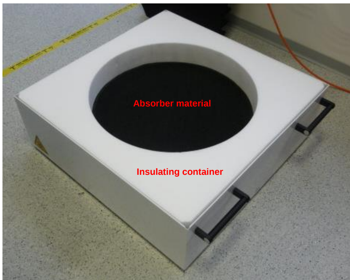
LN2 calibration target without the lid.
