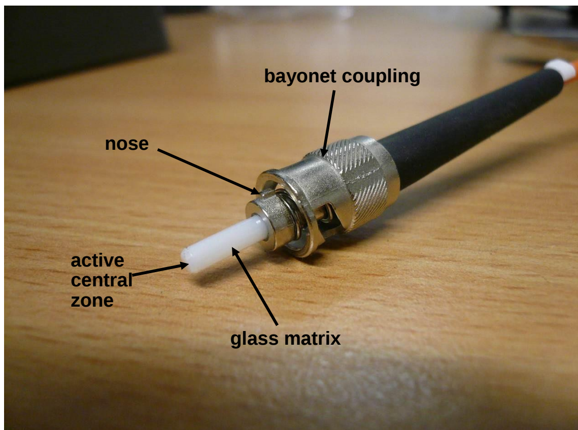
Details of the glass fiber connector.
