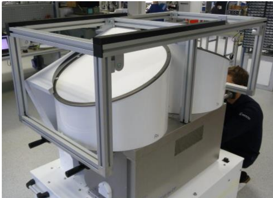
The radar with the properly mounted frame.
