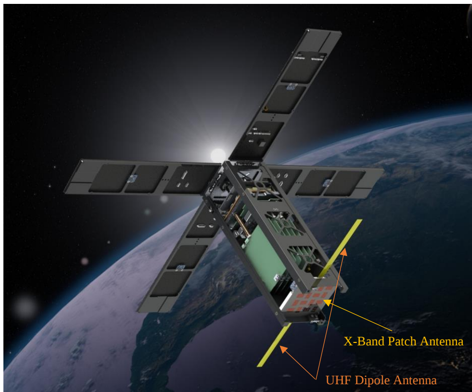
Figure 1: SPACE HAUC In Orbit (Artist Rendering)
