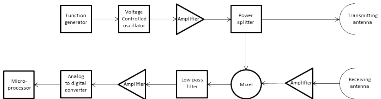
Figure 1. Radar block diagram.
