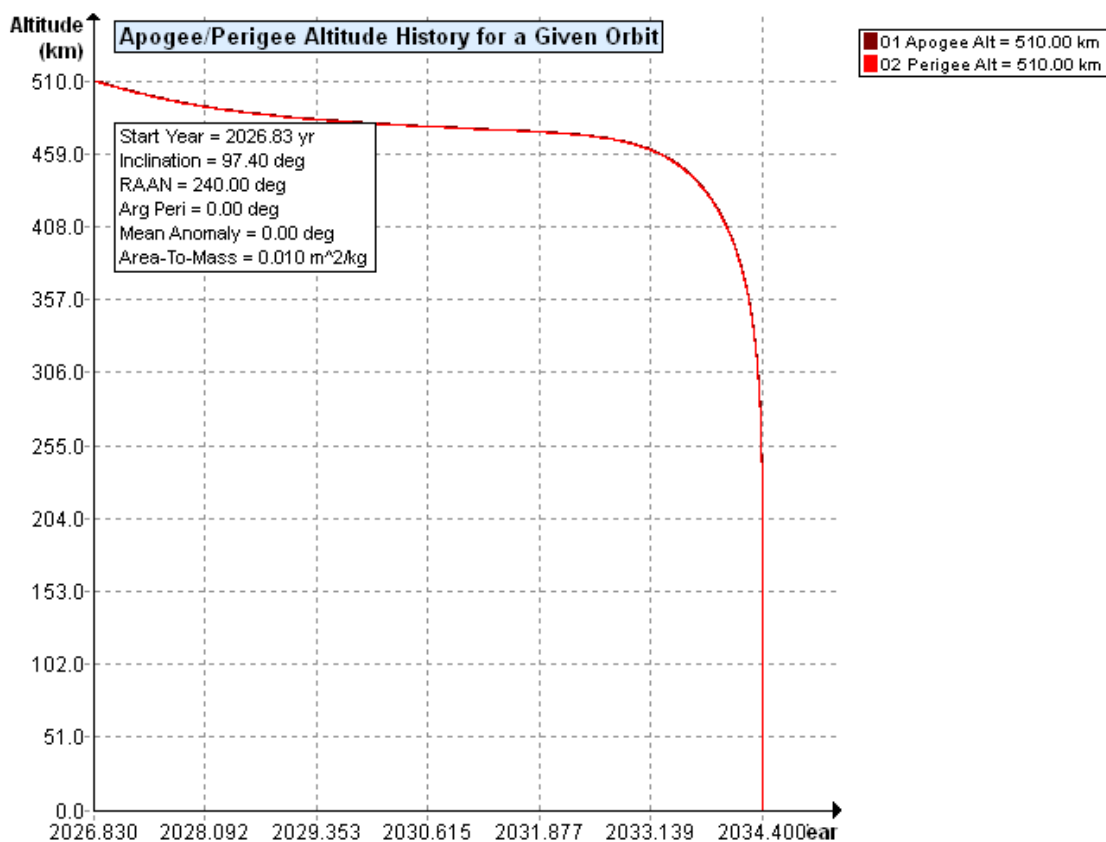
Figure 2 - SPRITE Deployed Configuration Orbit Evolution from 510 km.
