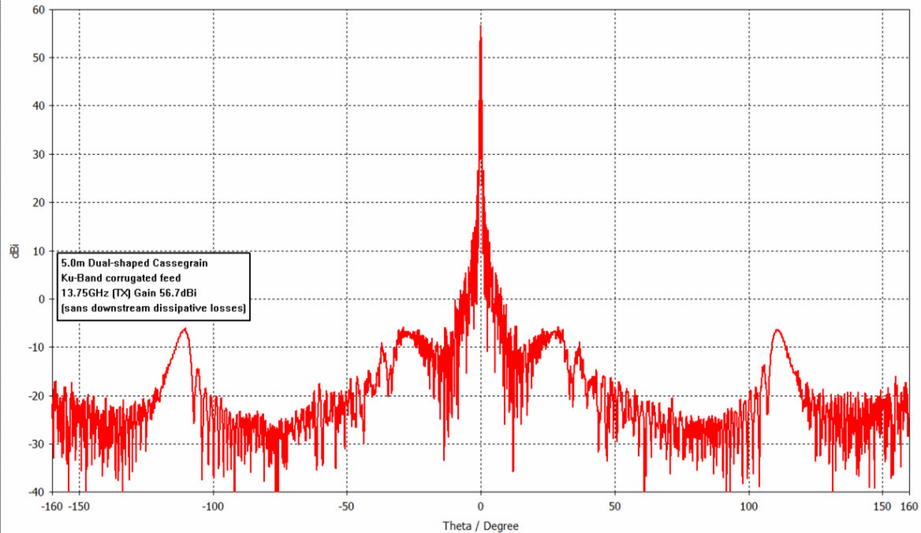
Farfield Directivity Abs (Phi=0)
