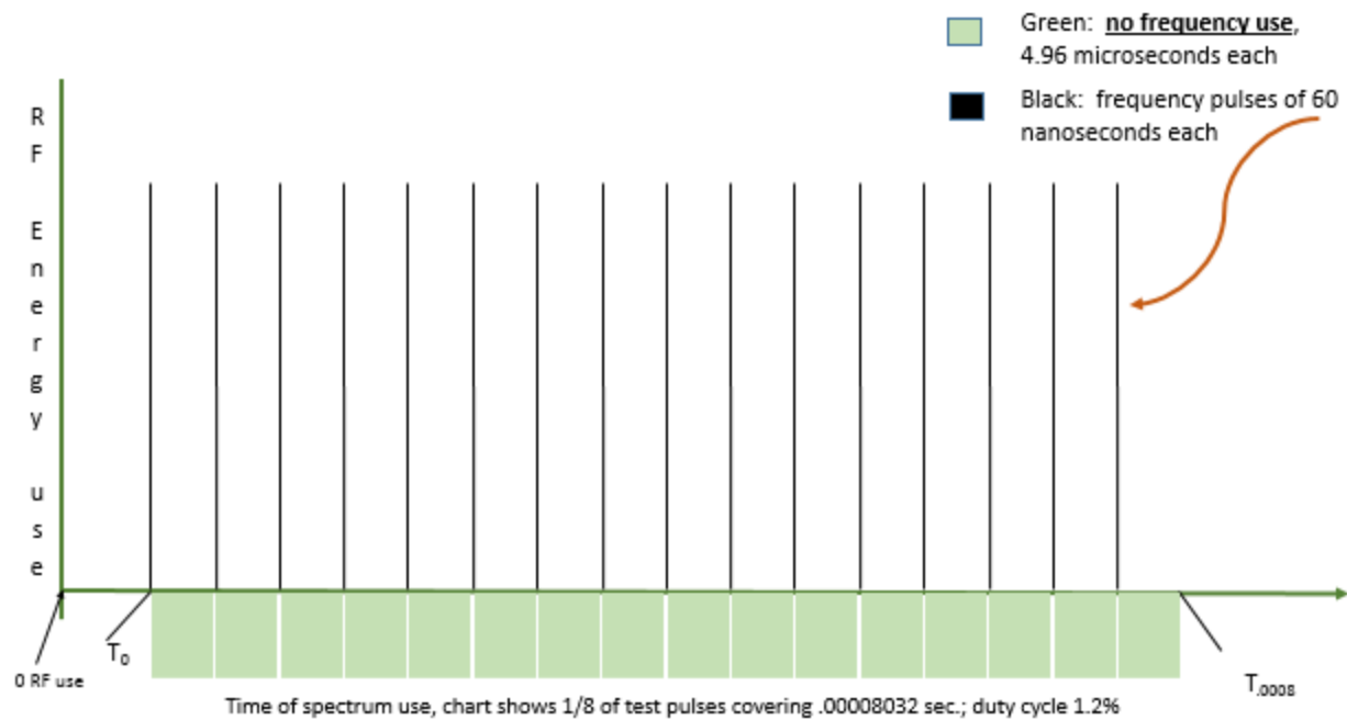
Figure 1. Illustration of Duty Cycle for 128 Pulses at a Frequency
