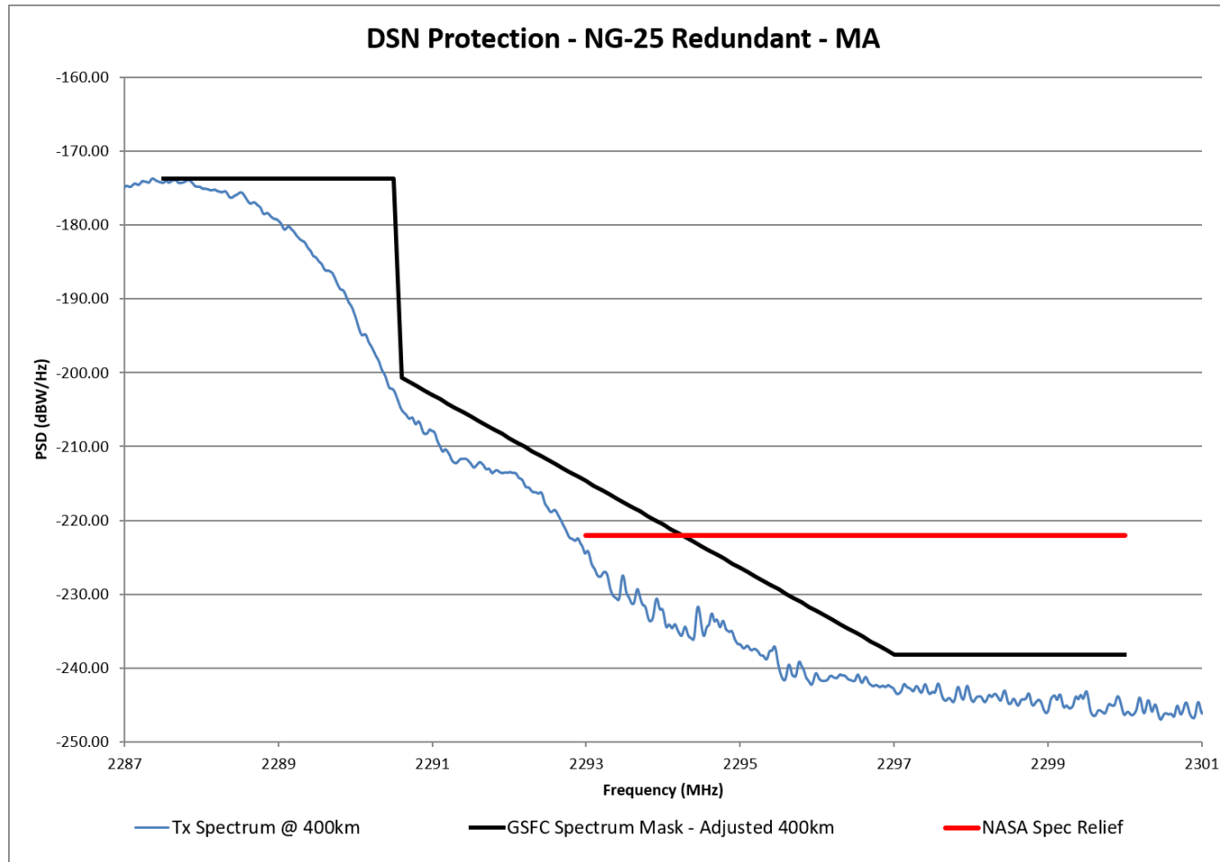
Figure 5. DSN Performance for TDRS Return Link 6M16G1D, ERP=7.55 W, Range = 400 km, Redundant Transmitter (CTC-B)
