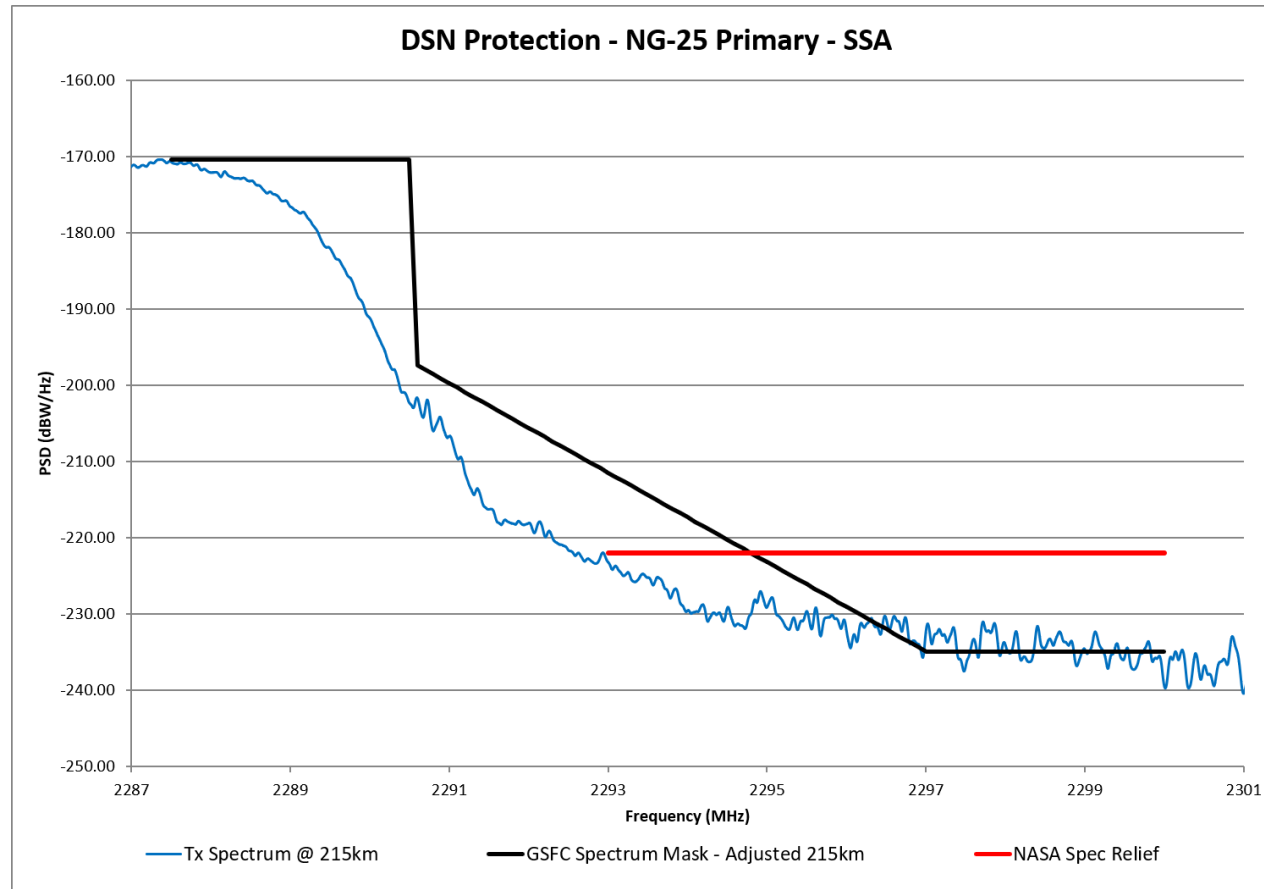
Figure 2. DSN Performance for TDRS Return Link 6M16G1D, ERP = 4.53 W, Range = 215 km, Primary Transmitter (CTC-A)
