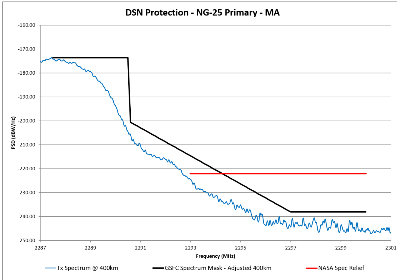
Figure 4. DSN Performance for TDRS Return Link 6M16G1D, ERP = 7.55 W, Range = 400 km, Primary Transmitter (CTC-A)
