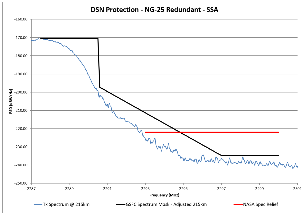
Figure 3. DSN Performance for TDRS Return Link 6M16G1D, ERP=4.53 W, Range = 215 km, Redundant Transmitter (CTC-B)
