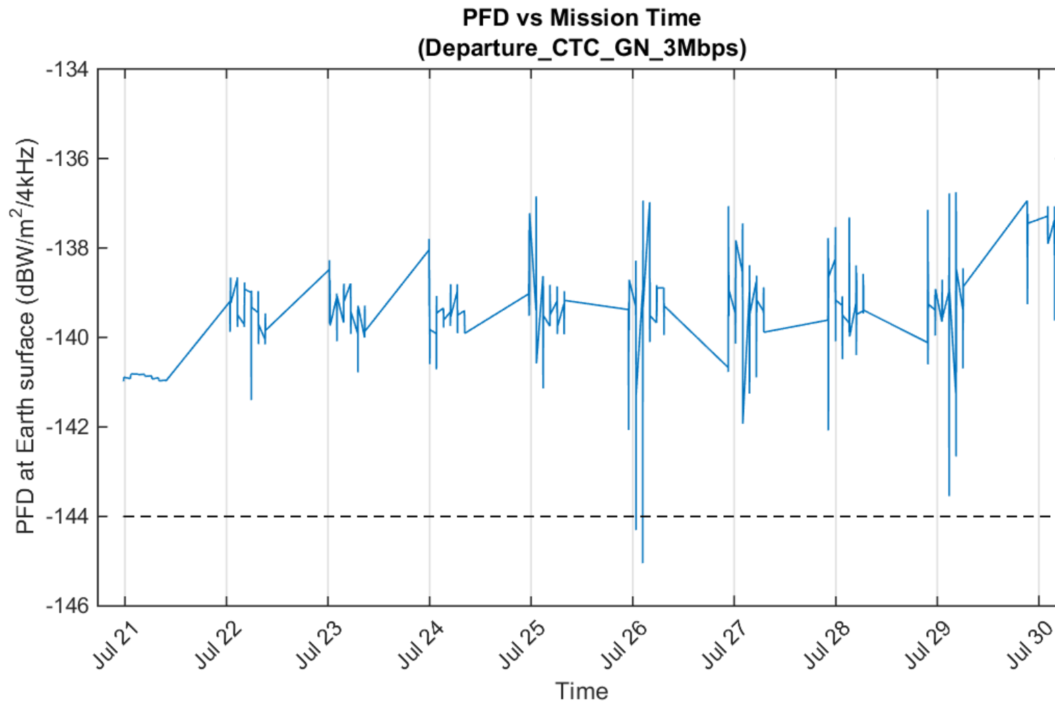
Figure 13 NG-11 Cygnus PFD During Departure Phase (3M00G1D Emitter – GN 3 Mbps)
