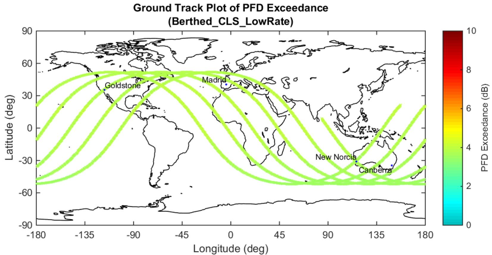
Figure 22 NG-11 Cygnus PFD Limit Exceedance During Mission Berthed (5M93G1D Emitter)
