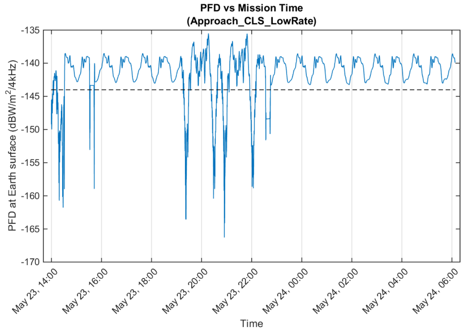
Figure 5 NG-11 Cygnus PFD During Mission Nominal Approach (5M93G1D Emitter)
