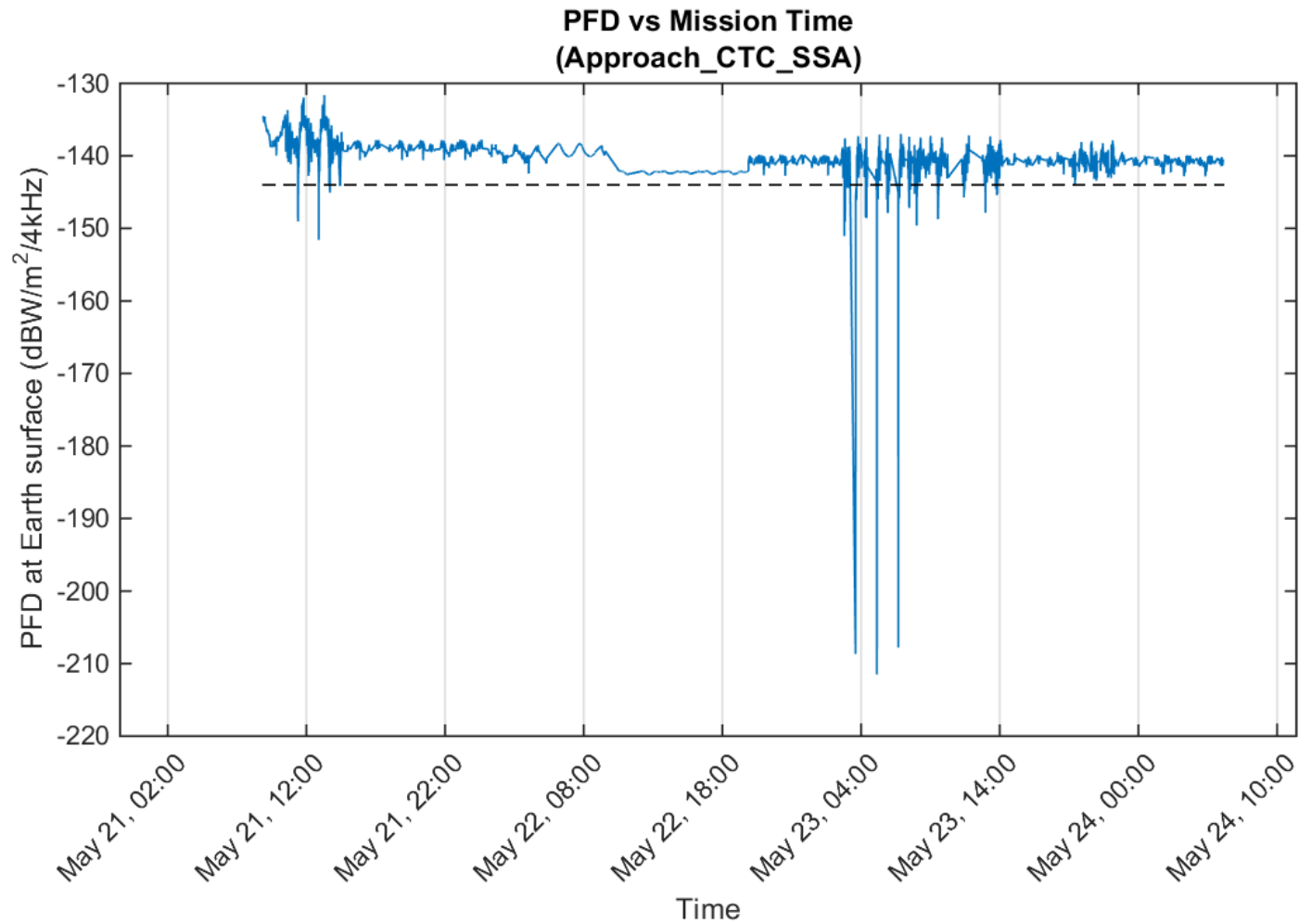
Figure 1 NG-11 Cygnus PFD During Mission Nominal Approach TDRS SSA (6M16G1D Emitter)
