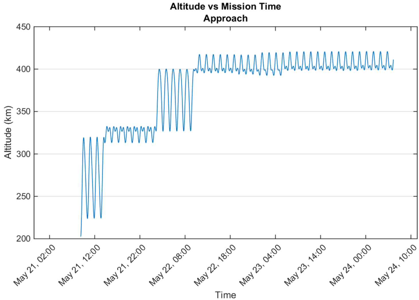
Figure 15 NG-11 Cygnus Altitude vs. Mission Time (Approach)
