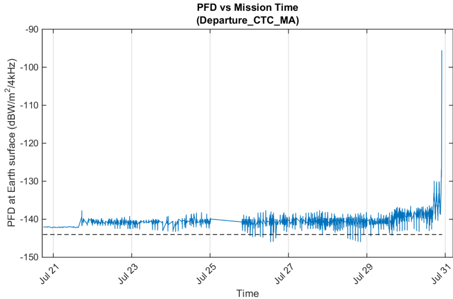
Figure 11 NG-11 Cygnus PFD During Departure Phase (6M16G1D Emitter – TDRS MA)
