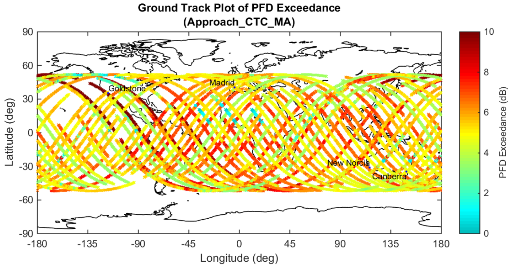
Figure 18 NG-11 Cygnus PFD Limit Exceedance During Mission Approach TDRS MA (6M16G1D Emitter)
