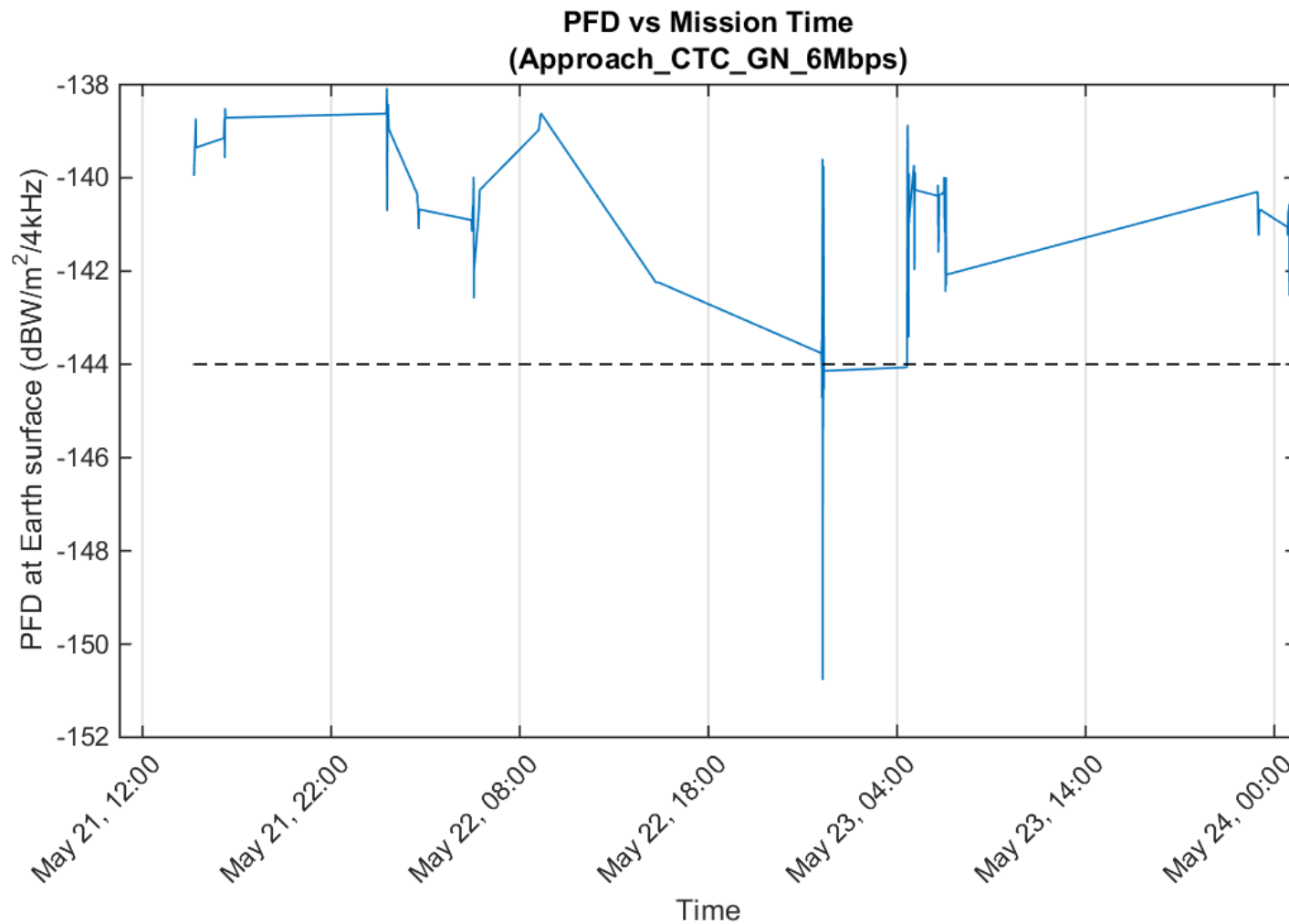
Figure 3 NG-11 Cygnus PFD During Mission Nominal Approach (4M98G1D Emitter)
