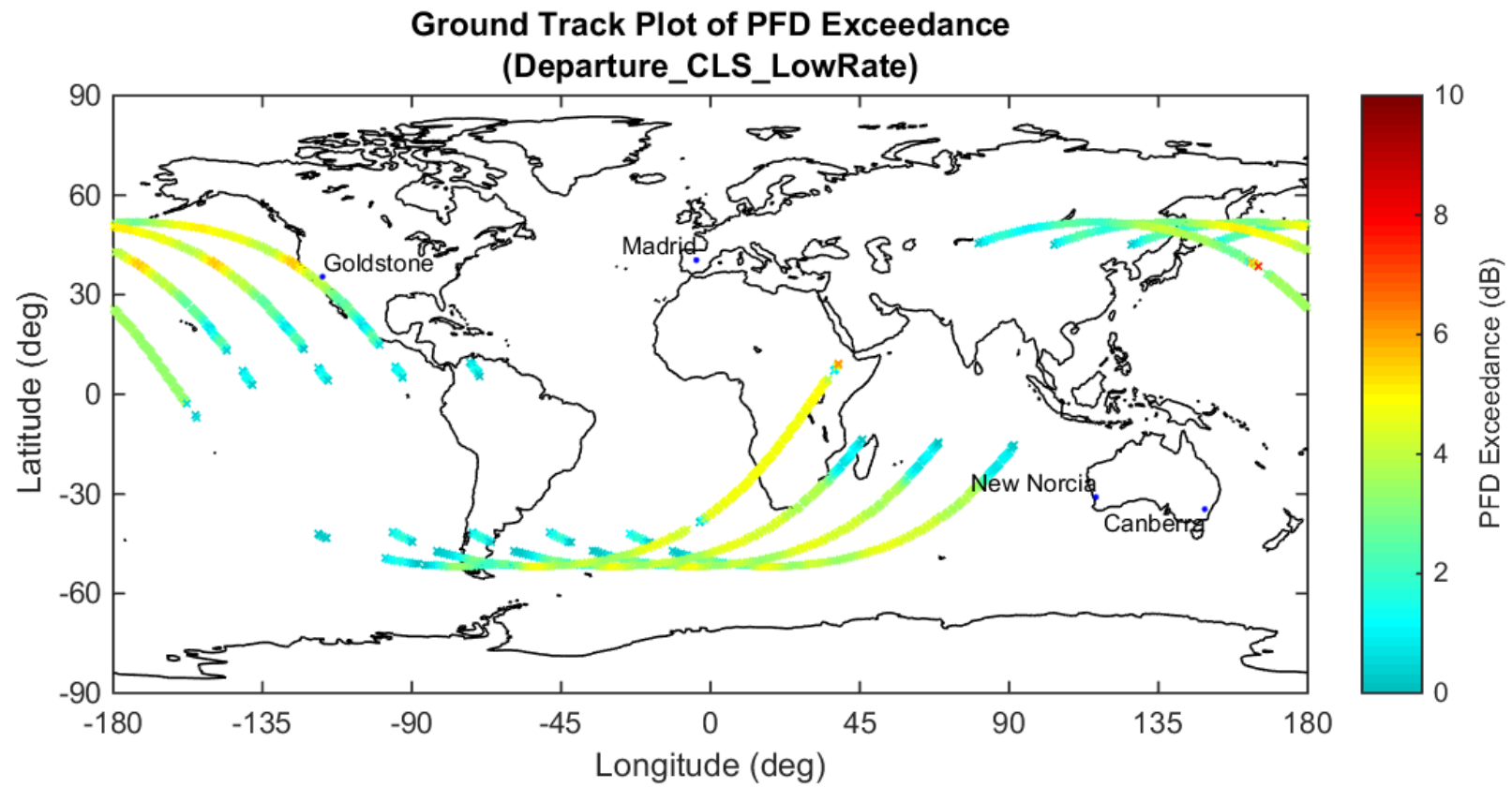
Figure 27 NG-11 Cygnus PFD Limit Exceedance During Mission Departure (5M93G1D Emitter)
