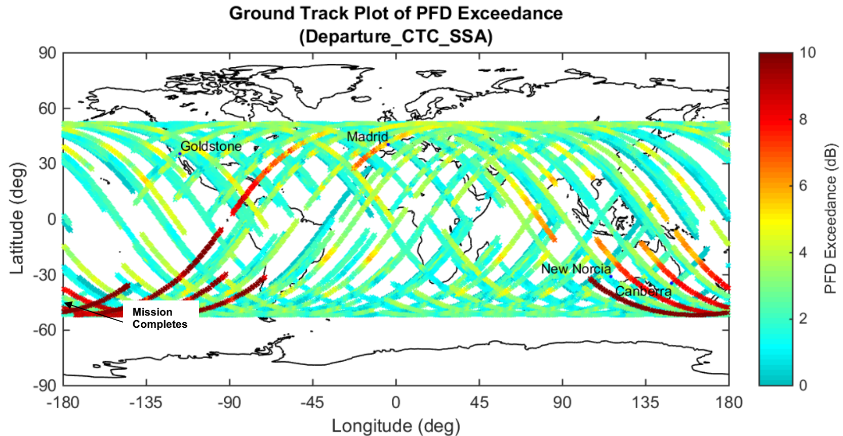
Figure 23 NG-11 Cygnus PFD Limit Exceedance During Mission Departure (6M16G1D Emitter – TDRS SSA)
