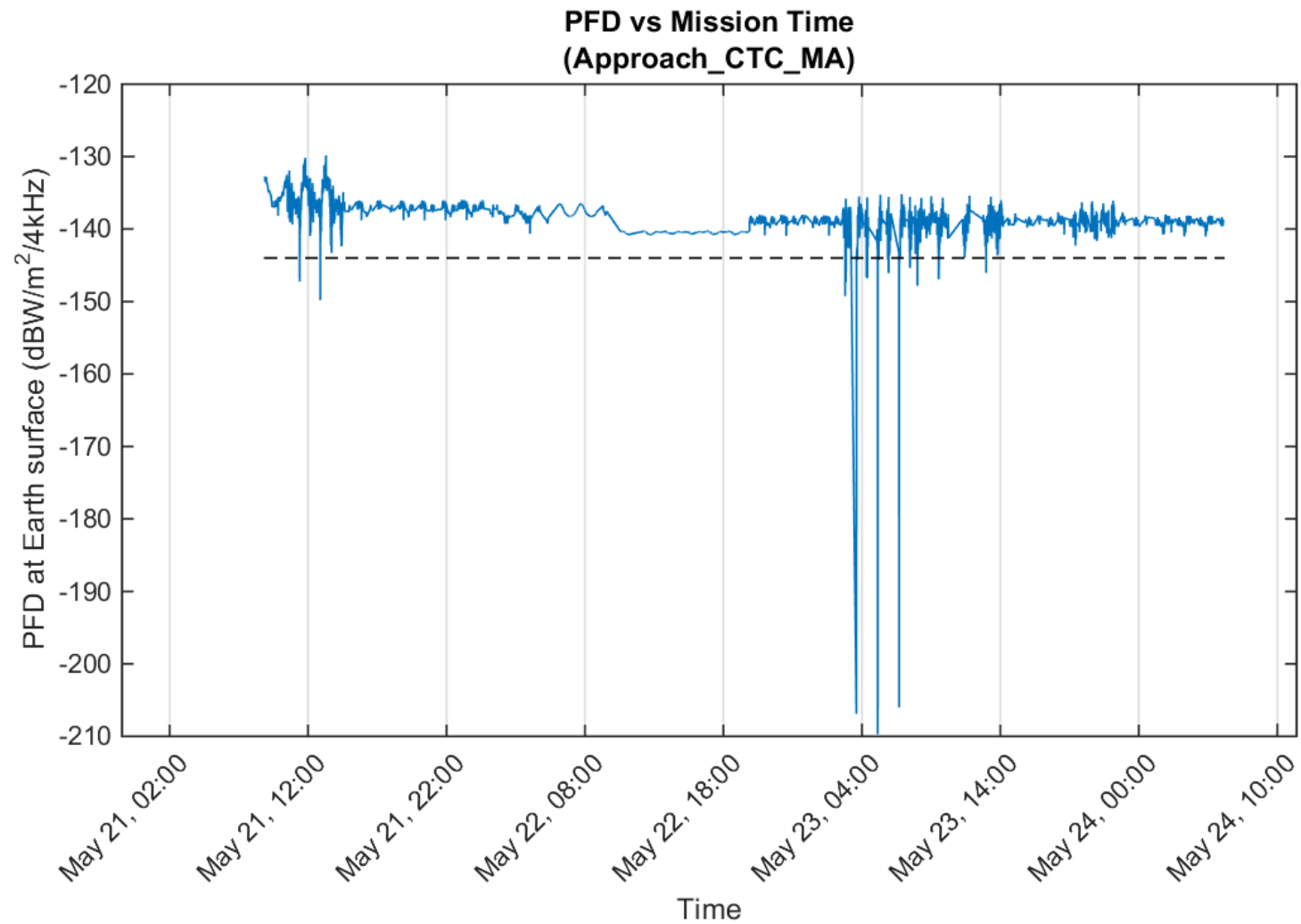
Figure 2 NG-11 Cygnus PFD During Mission Nominal Approach TDRS MA (6M16G1D Emitter)
