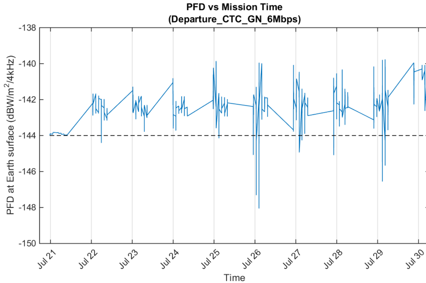
Figure 12 NG-11 Cygnus PFD During Departure Phase (4M98G1D Emitter – GN 6 Mbps)
