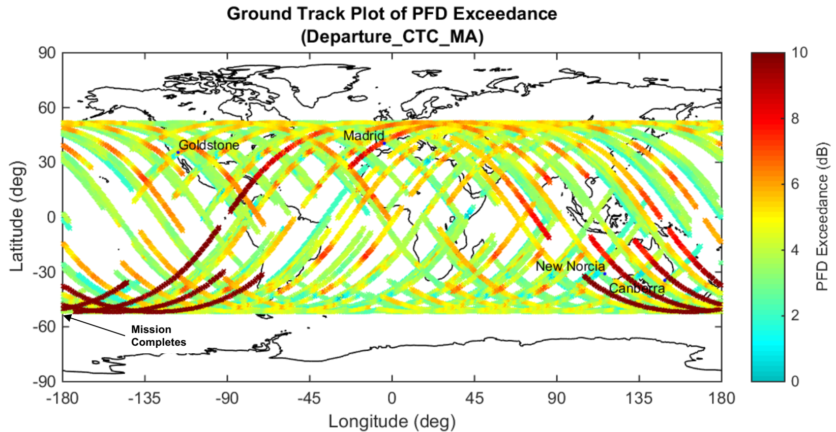
Figure 24 NG-11 Cygnus PFD Limit Exceedance During Mission Departure (6M16G1D Emitter – TDRS SMA)
