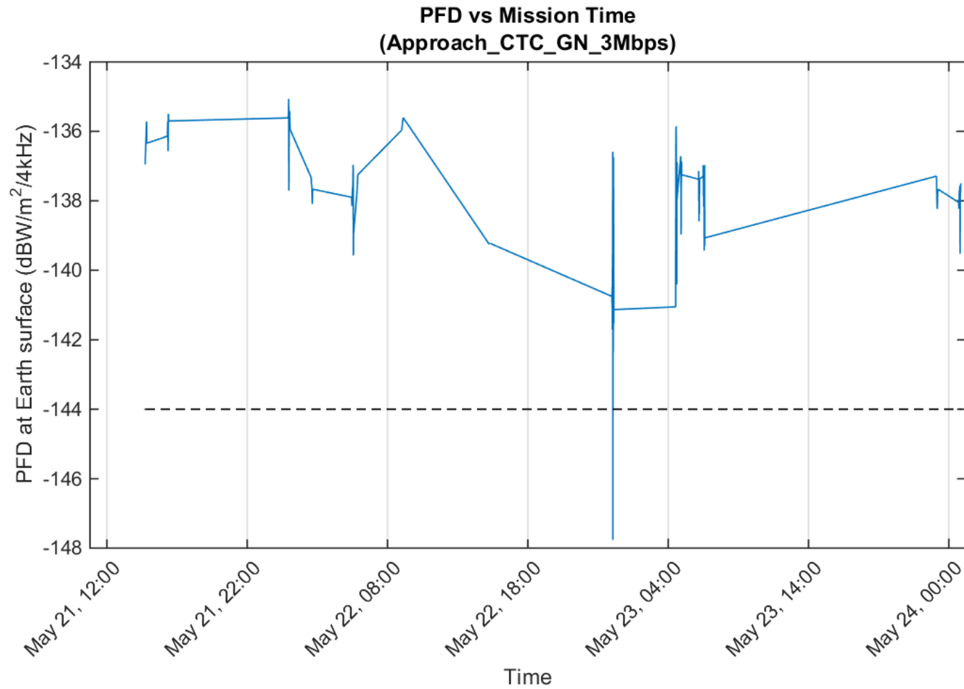
Figure 4 NG-11 Cygnus PFD During Mission Nominal Approach (3M00G1D Emitter)
