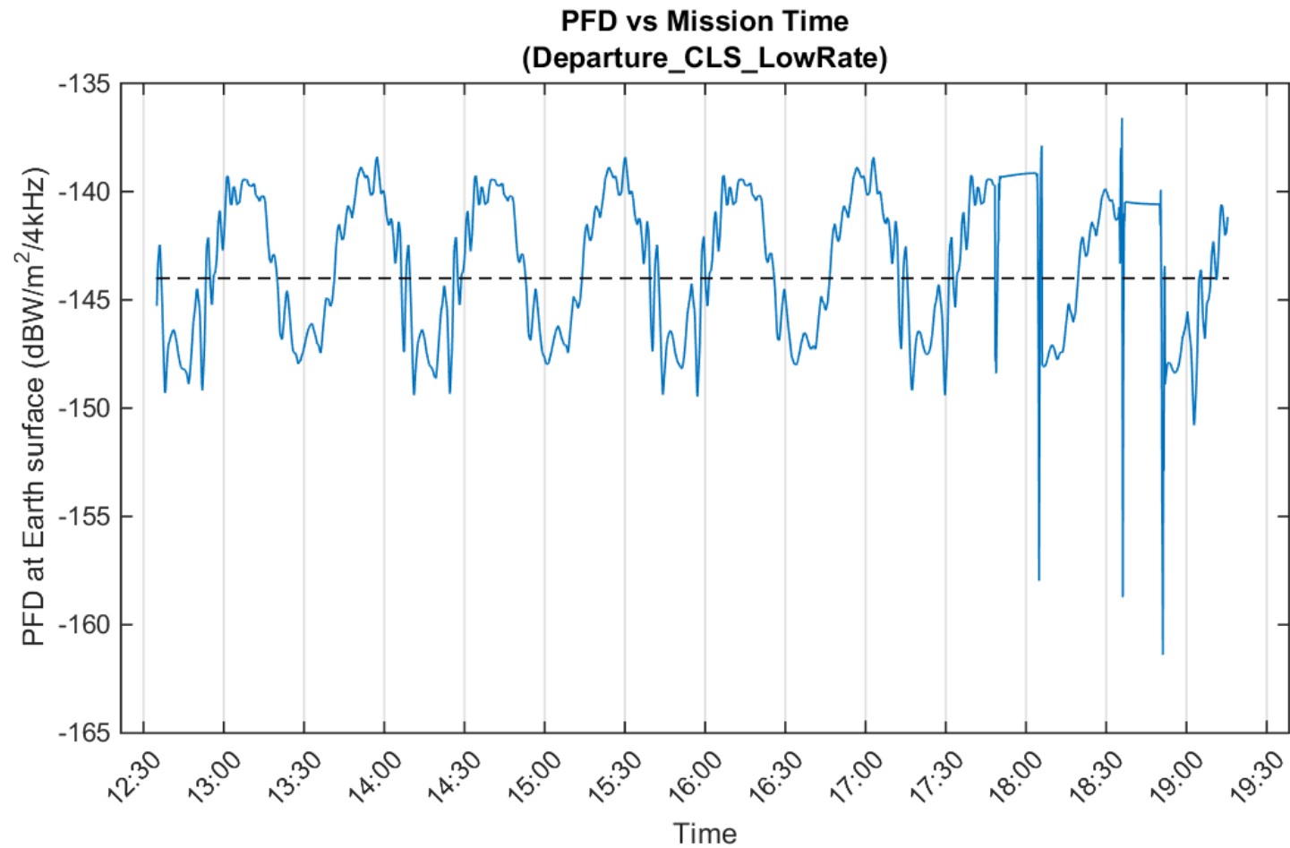
Figure 14 NG-11 Cygnus PFD During Departure Phase (5M93G1D Emitter)
