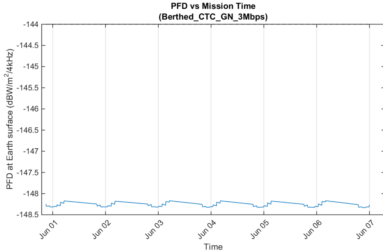
Figure 7 NG-11 Cygnus PFD During Berthed Phase (3M00G1D Emitter – GN 3 Mbps)
