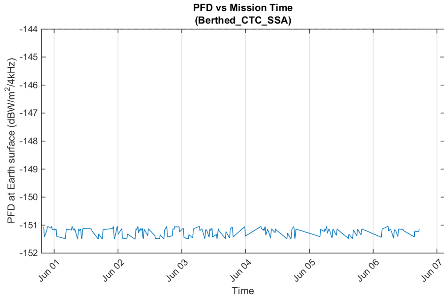
Figure 6 NG-11 Cygnus PFD During Berthed Phase (6M16G1D Emitter – TDRS SSA)
