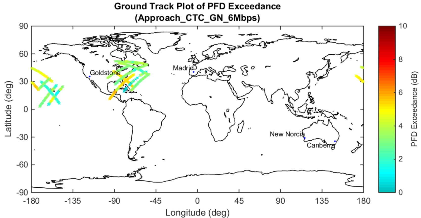
Figure 19 NG-11 Cygnus PFD Limit Exceedance During Mission Approach (4M98G1D Emitter GN 6 Mbps)
