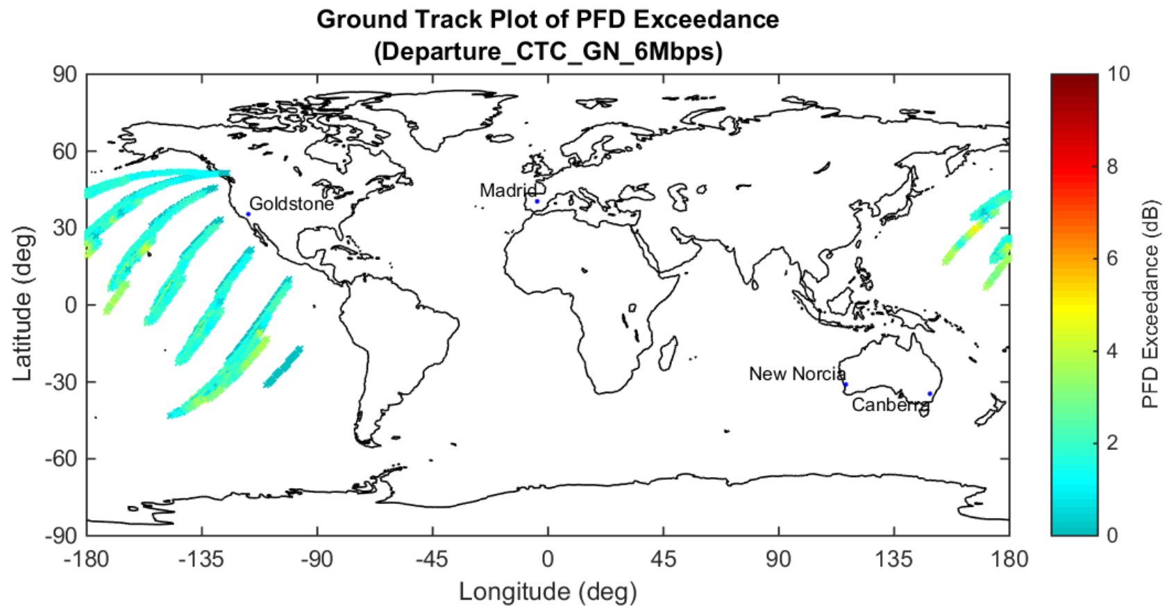
Figure 25 NG-11 Cygnus PFD Limit Exceedance During Mission Departure (4M98G1D Emitter – GN 6 Mbps)
