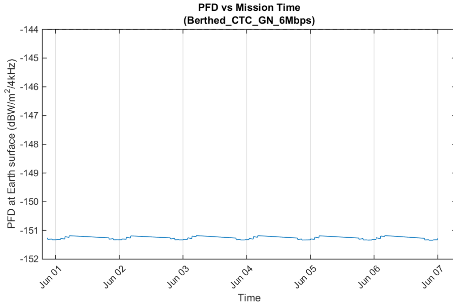
Figure 8 NG-11 Cygnus PFD During Berthed Phase (4M98G1D Emitter – GN 6 Mbps)
