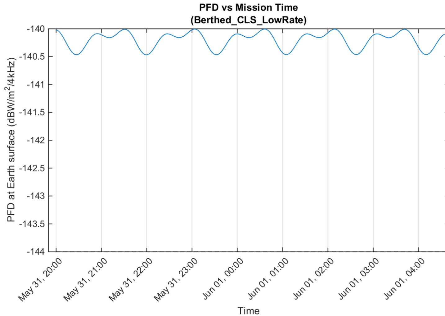
Figure 9 NG-11 Cygnus PFD During Berthed Phase (5M93G1D Emitter)
