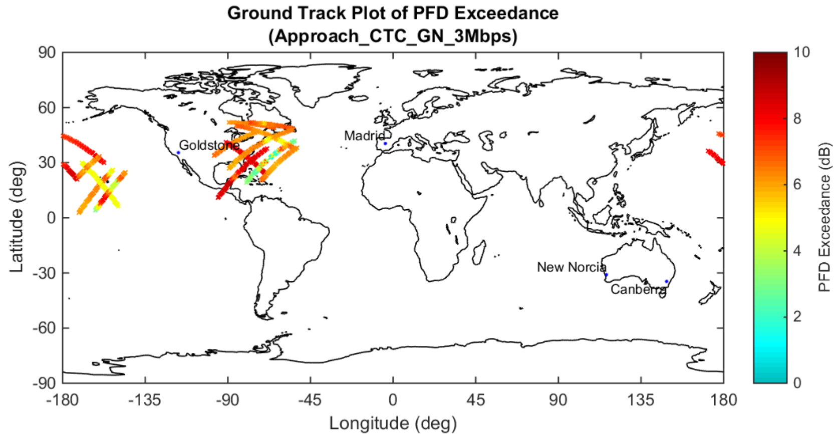
Figure 20 NG-11 Cygnus PFD Limit Exceedance During Mission Approach (3M00G1D Emitter GN 3 Mbps)
