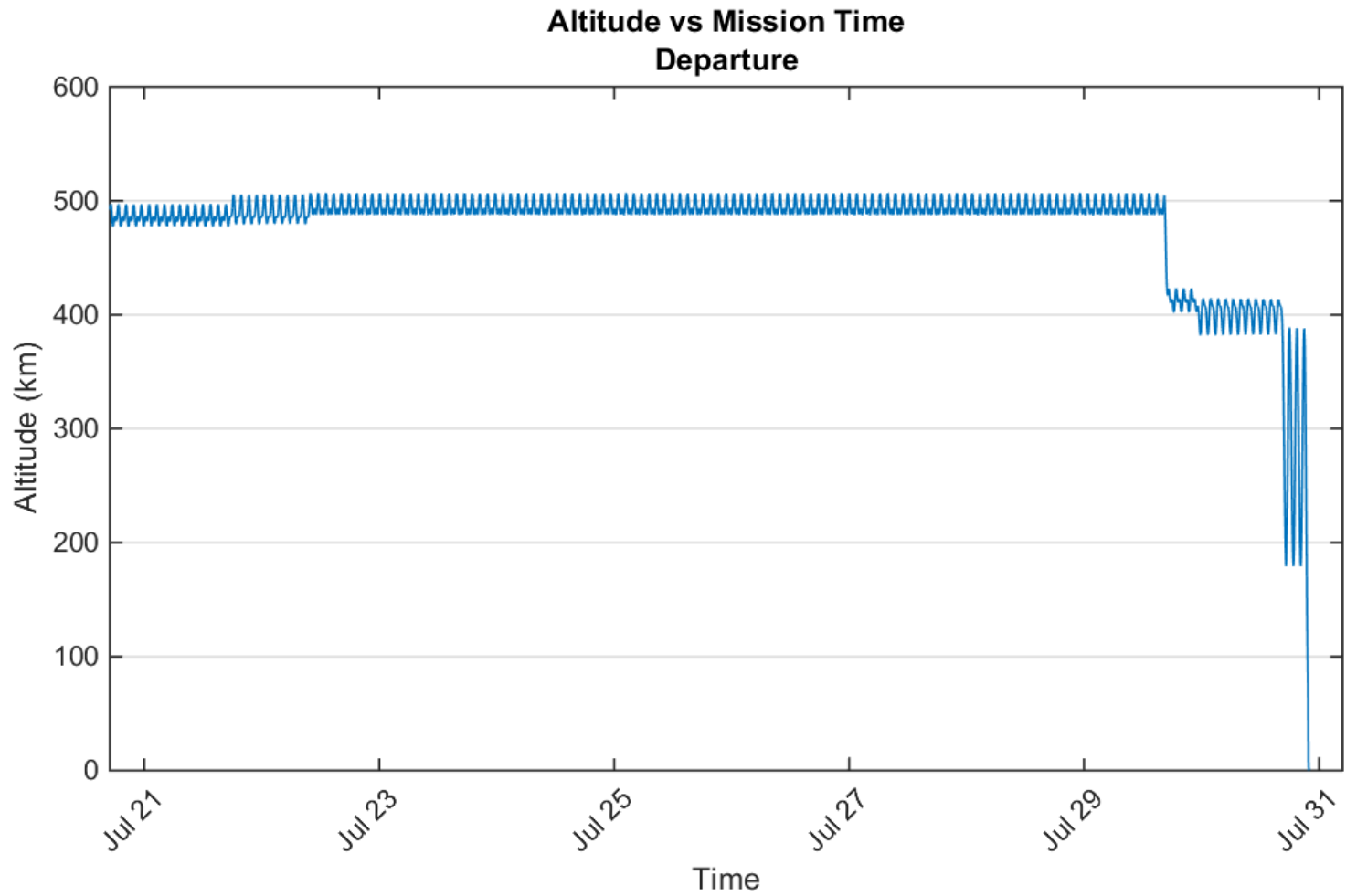
Figure 16 NG-11 Cygnus Altitude vs. Mission Time (Departure)
