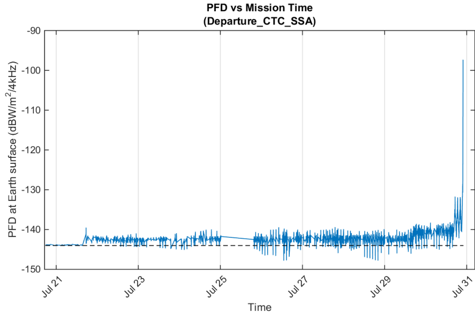
Figure 10 NG-11 Cygnus PFD During Departure Phase (6M16G1D Emitter – TDRS SSA)
