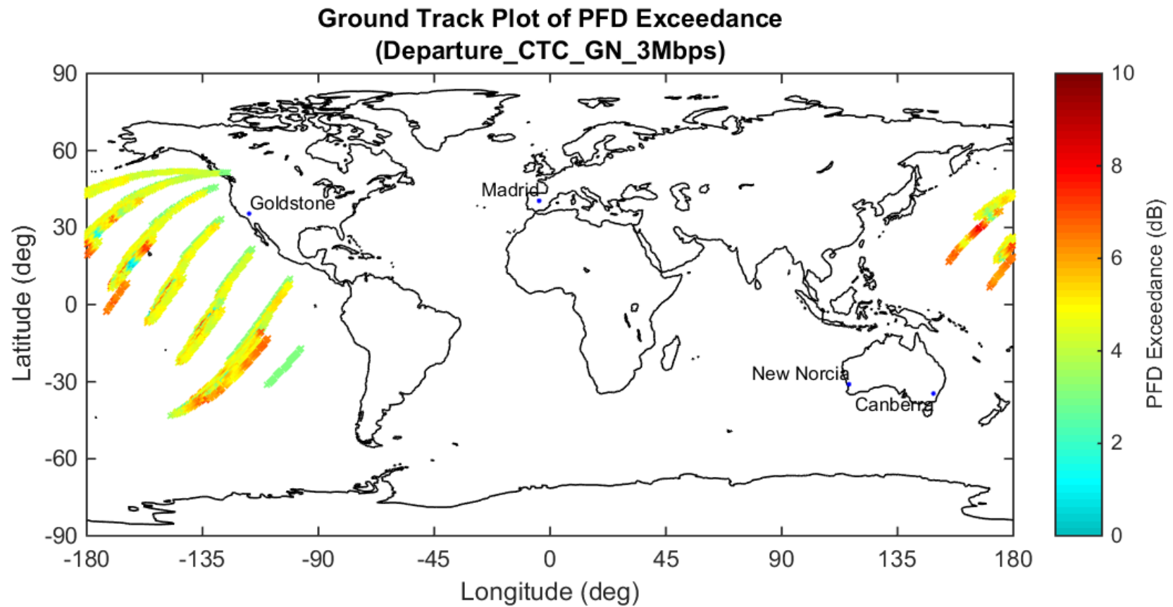
Figure 26 NG-11 Cygnus PFD Limit Exceedance During Mission Departure (3M00G1D Emitter – GN 3 Mbps)
