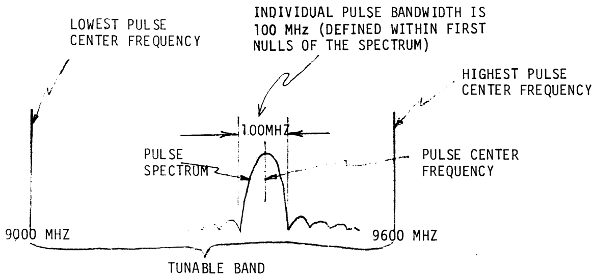
FIGURE 2 NECESSARY BANDWIDTH
