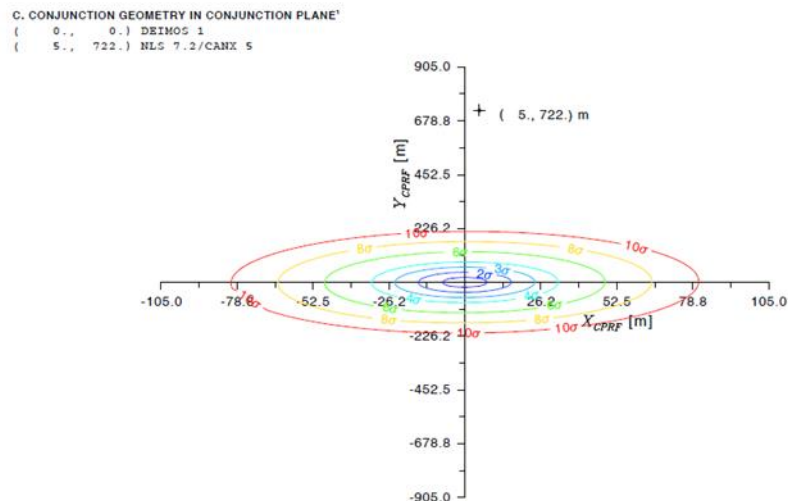
Figure 3. Example of 2D conjunction plane.
