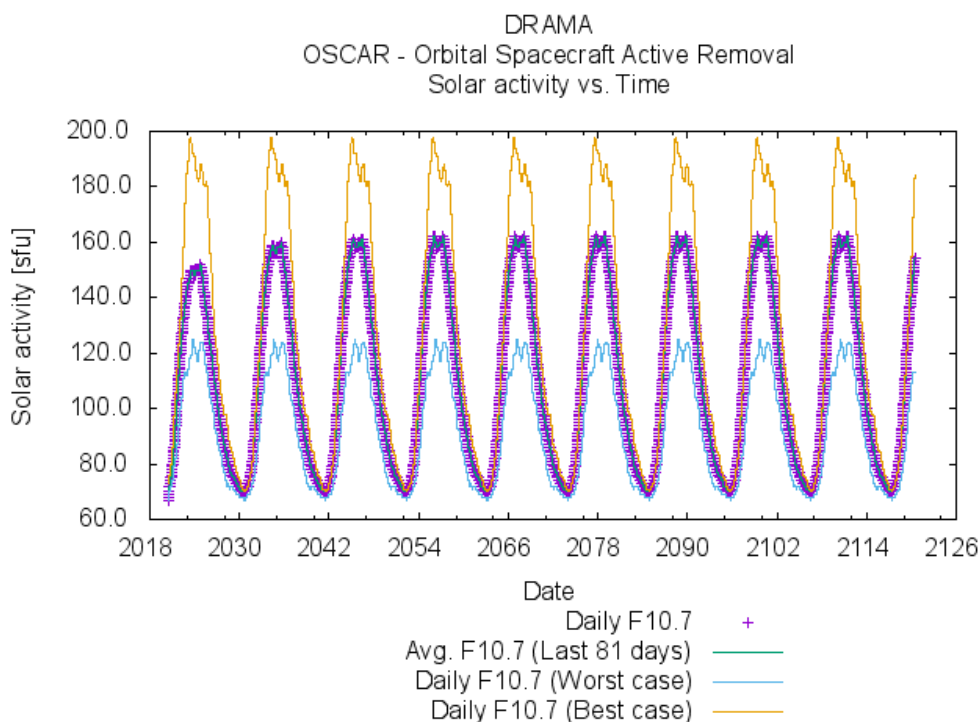
Figure. 1: Solar cycles.
