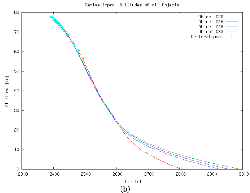
Figure 5-3: (a) Altitude vs distance and (b) altitude vs time of the fragmentation of the Deimos-2 spacecraft predicted with the ESA tool DRAMA/SARA.
