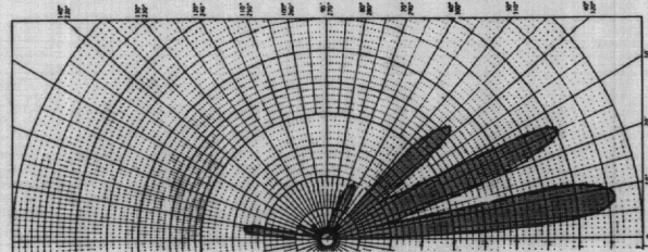
Frequency 30.0 MHz
