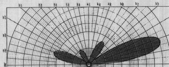
Frequency 12.5 MHz
