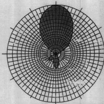
Frequency 30.0 MHz 60° HP Beam Width
