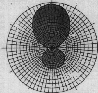
Frequency 12.5 MHz 70° HP Beam Width
