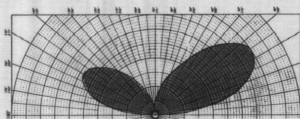
Frequency 6.2 MHz
