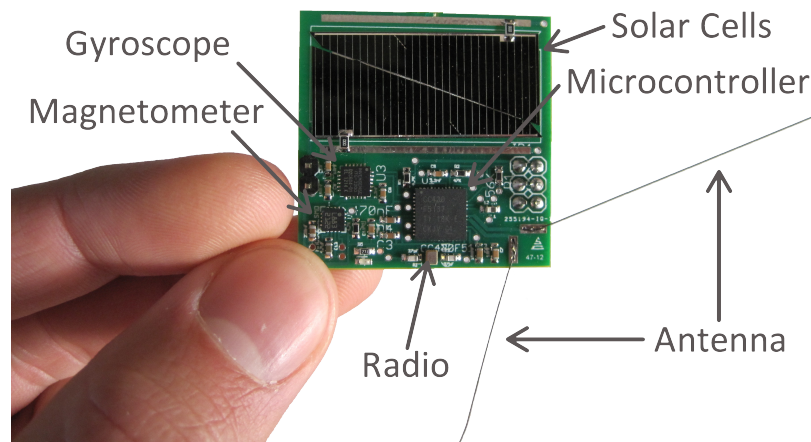
Figure 1: Sprite Spacecraft
