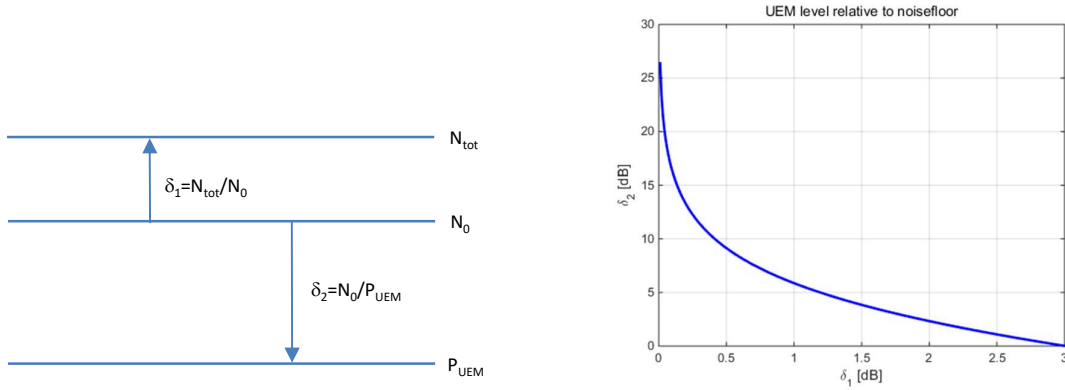
Figure K-1: Relative noise measurement
