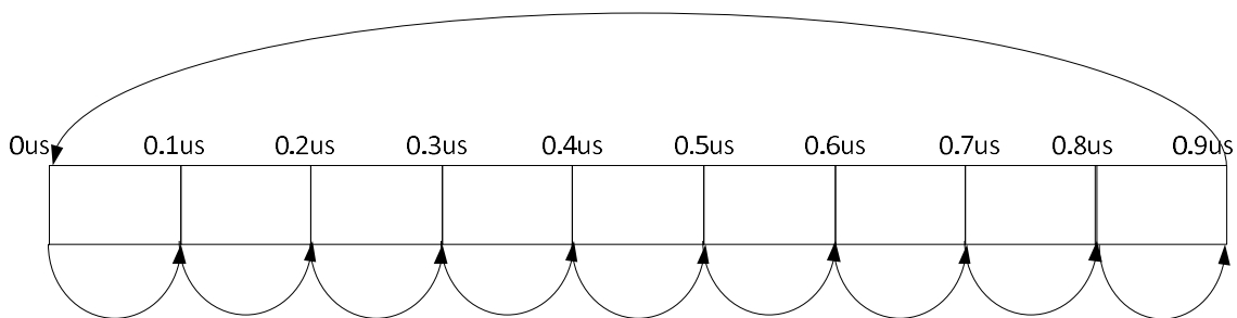
Figure 8.4.1.4.2-2: Timing offset scheme for PRACH preamble format 0
