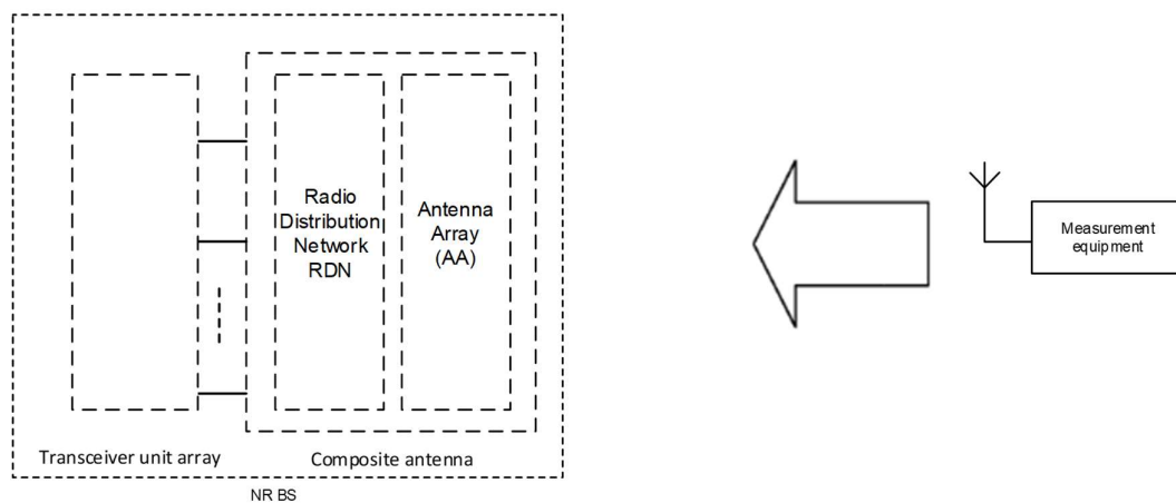
Figure 4.5.2-1: Receiver test interfaces
