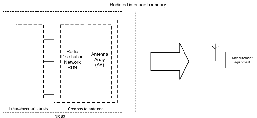
Figure 4.5.1-1: Transmitter test interfaces
