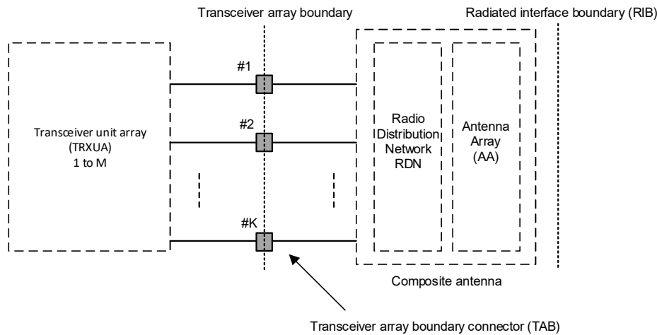
Figure 4.2-1: General architecture of BS type 1-H
