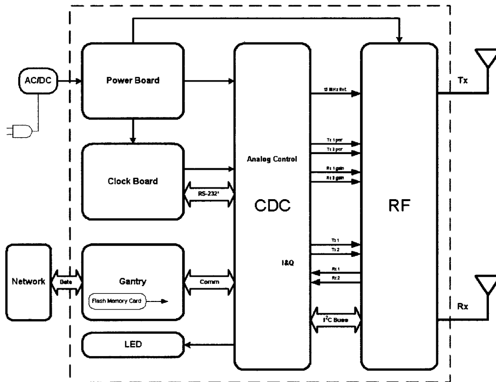
Simplified Block Diagram of Pico-BTS
