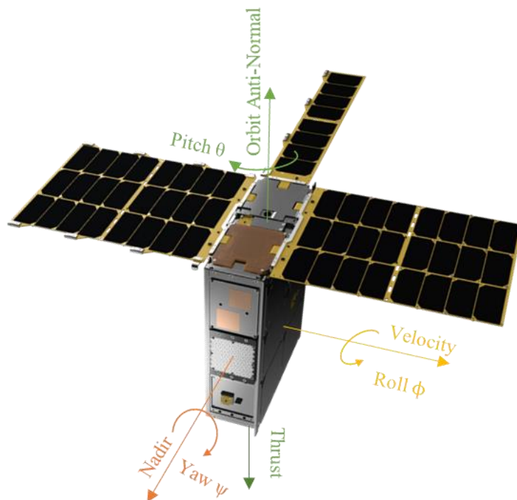
Figure 2: Cesium Spacecraft in normal operation mode
