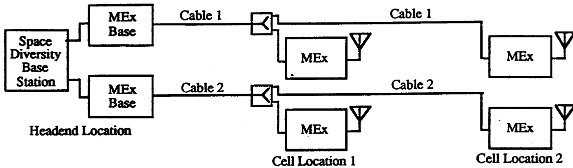
Figure A2. -- Space diversity test setup.
