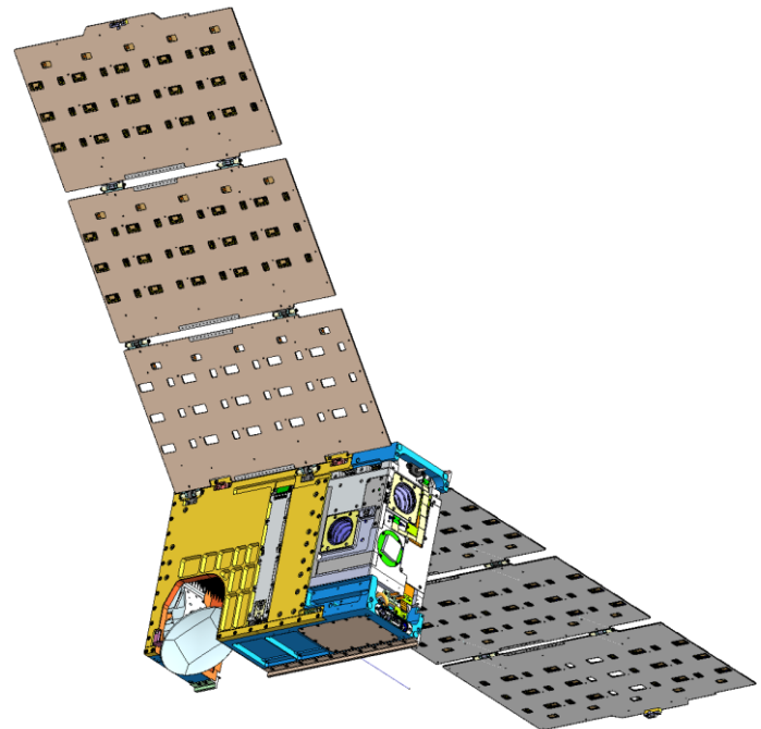
Figure 1. TEMPEST-D Spacecraft with Solar Panels and UHF antenna deployed.
