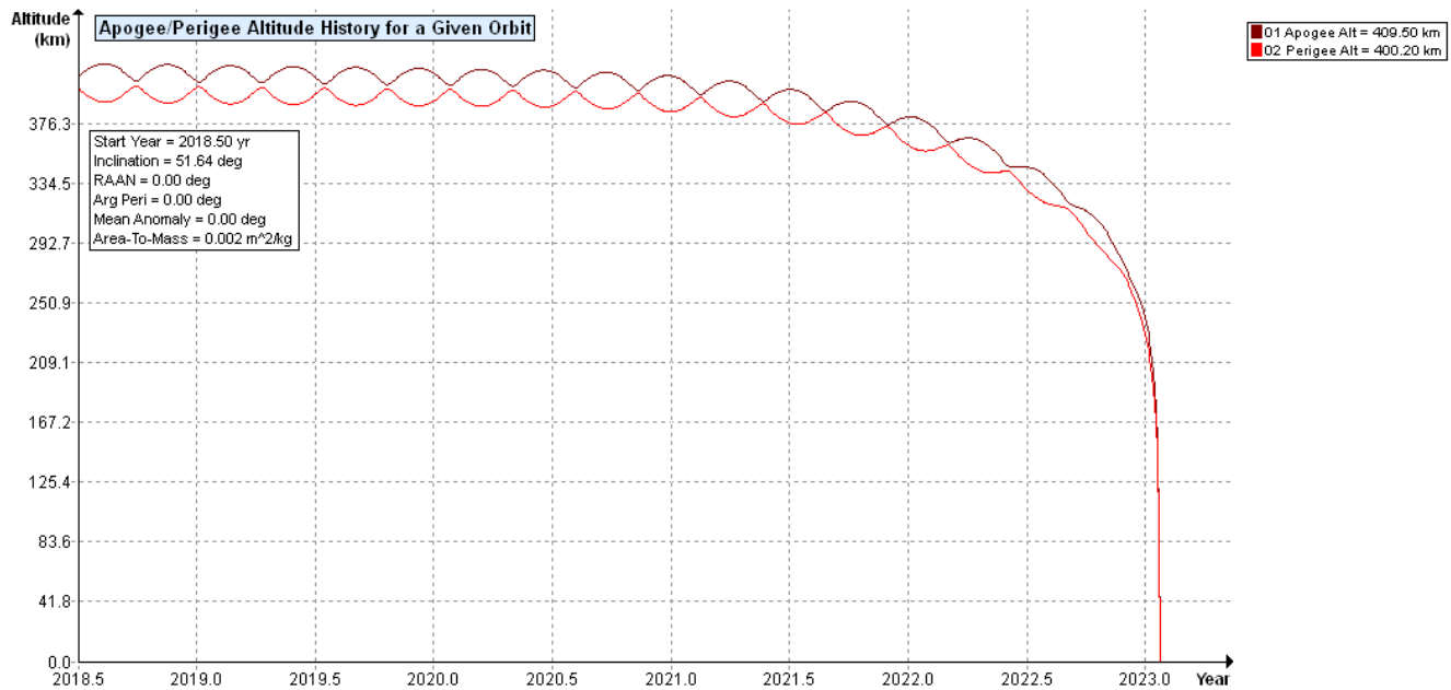
Figure 2. TEMPEST-D Orbit Lifetime/Dwell Time and Orbit Decay
