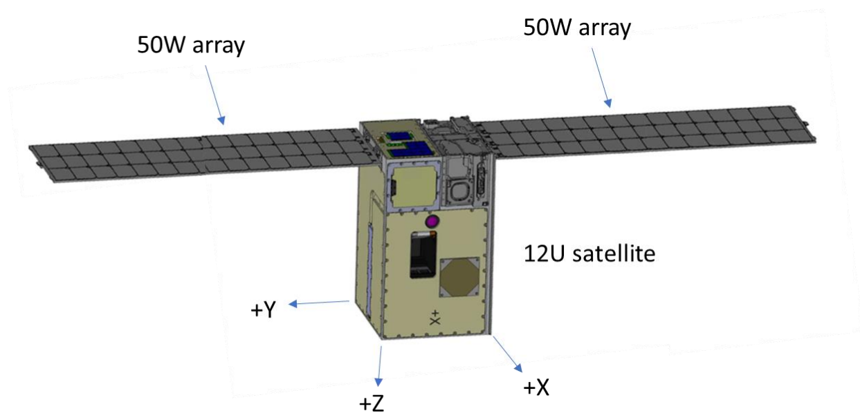
Figure 1: Slingshot-1 spacecraft shown with solar arrays deployed. CBE mass is 19.2 kg. Deployed outer dimensions are 140 x 37 x 22 cm.
