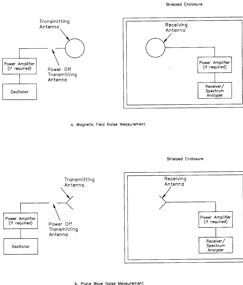
FIG. 4 Noise Measurement Procedures
